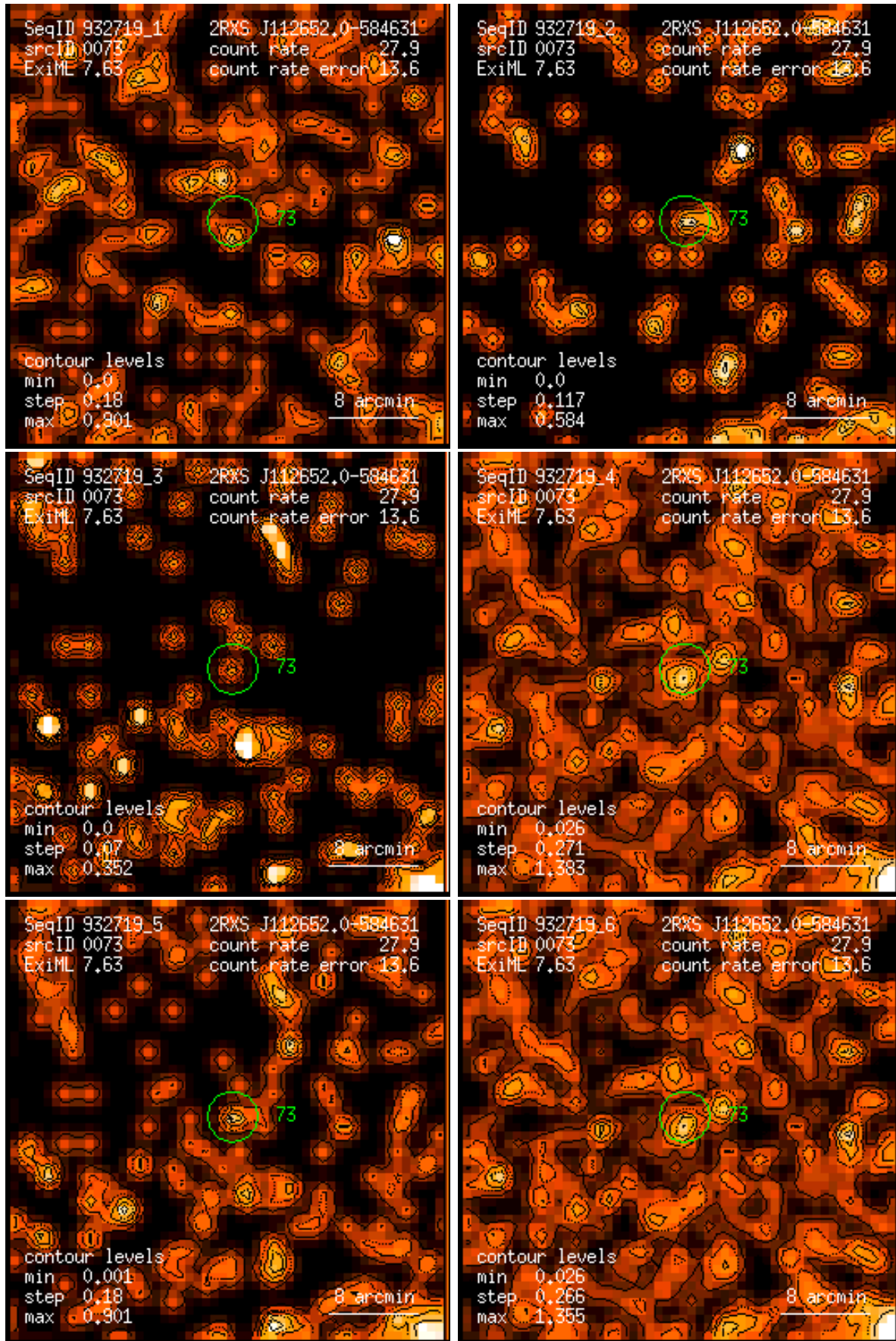
Figure 73: RASS 932719: detection 0073: band rate images, Gaussian filter: (1) PSPC channels 11 – 41, (2) 52 – 90, (3) 91 – 201, (4) 11 – 235, (5) 52 – 201, (6) 11 – 201. Broad band rates in counts/ks. Band rate contour levels in counts/ks/arcmin 2 .
