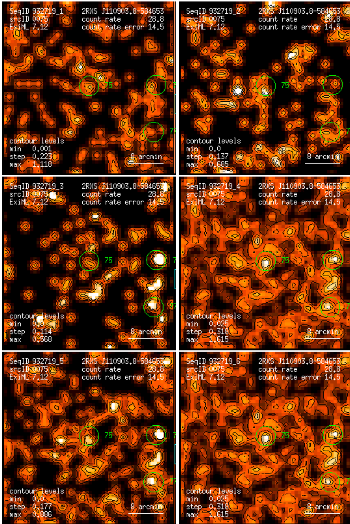
Figure 75: RASS 932719: detection 0075: band rate images, Gaussian filter: (1) PSPC channels 11 – 41, (2) 52 – 90, (3) 91 – 201, (4) 11 – 235, (5) 52 – 201, (6) 11 – 201. Broad band rates in counts/ks. Band rate contour levels in counts/ks/arcmin 2 .
