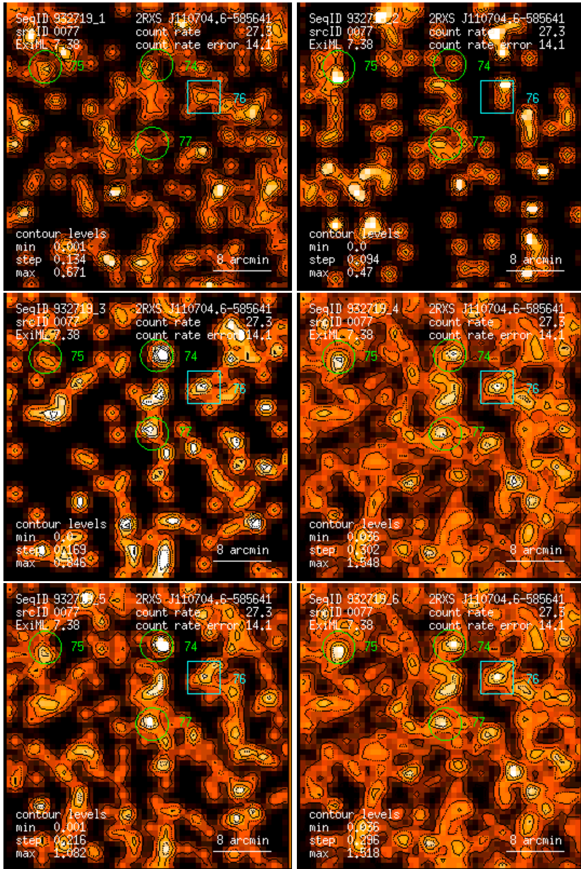
Figure 77: RASS 932719: detection 0077: band rate images, Gaussian filter: (1) PSPC channels 11 – 41, (2) 52 – 90, (3) 91 – 201, (4) 11 – 235, (5) 52 – 201, (6) 11 – 201. Broad band rates in counts/ks. Band rate contour levels in counts/ks/arcmin 2 .
