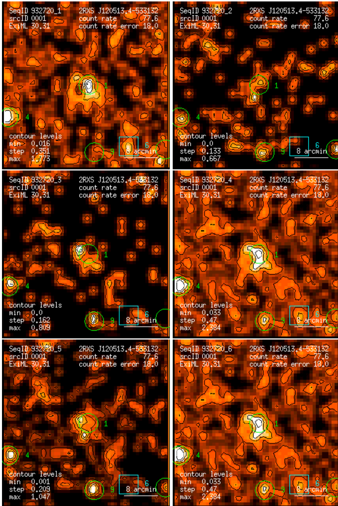
Figure 1: RASS 932720: detection 0001: band rate images, Gaussian filter: (1) PSPC channels 11 – 41, (2) 52 – 90, (3) 91 – 201, (4) 11 – 235, (5) 52 – 201, (6) 11 – 201. Broad band rates in counts/ks. Band rate contour levels in counts/ks/arcmin 2 .
