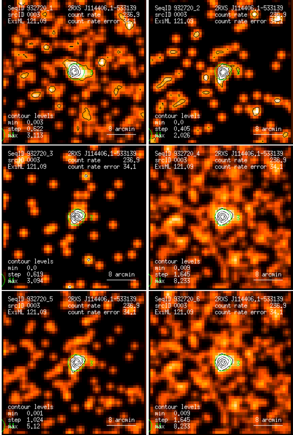
Figure 3: RASS 932720: detection 0003: band rate images, Gaussian filter: (1) PSPC channels 11 – 41, (2) 52 – 90, (3) 91 – 201, (4) 11 – 235, (5) 52 – 201, (6) 11 – 201. Broad band rates in counts/ks. Band rate contour levels in counts/ks/arcmin 2 .
