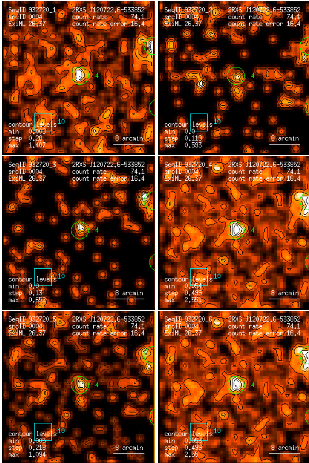
Figure 4: RASS 932720: detection 0004: band rate images, Gaussian filter: (1) PSPC channels 11 – 41, (2) 52 – 90, (3) 91 – 201, (4) 11 – 235, (5) 52 – 201, (6) 11 – 201. Broad band rates in counts/ks. Band rate contour levels in counts/ks/arcmin 2 .
