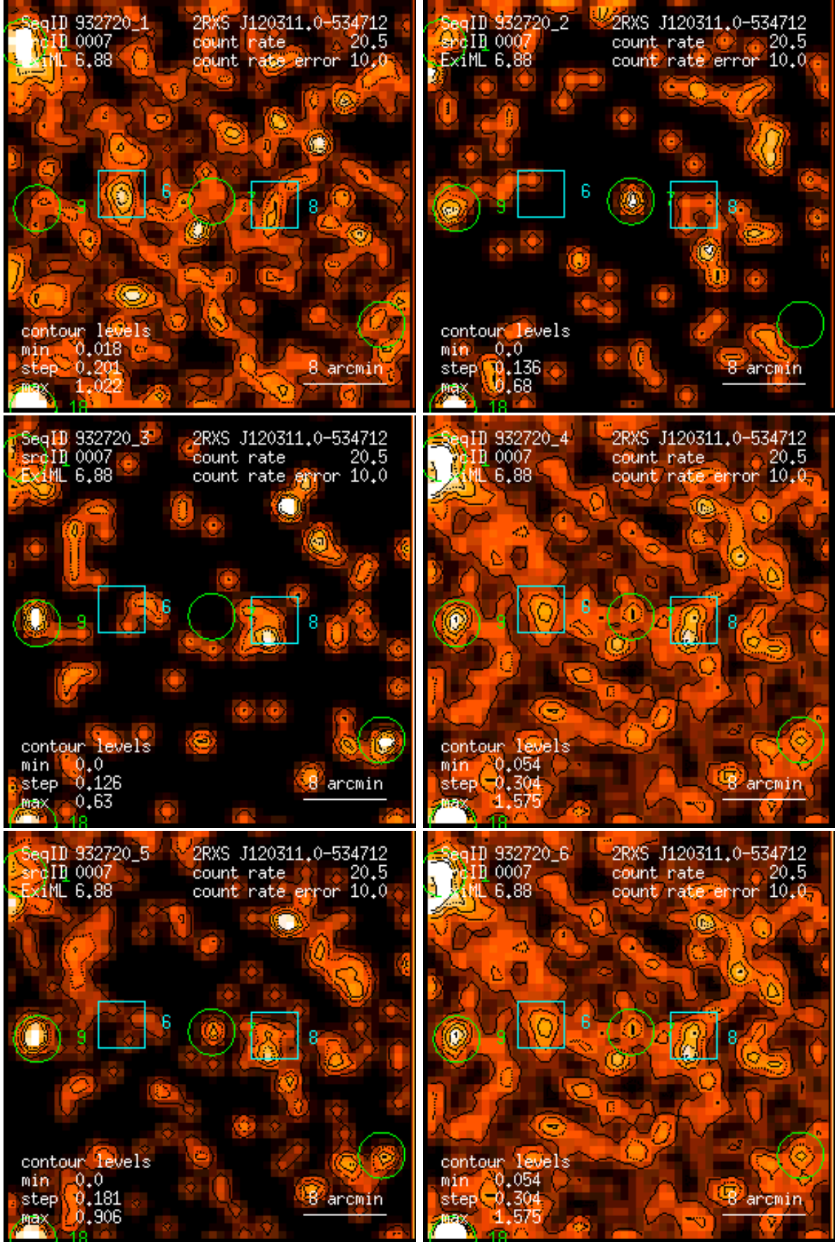
Figure 7: RASS 932720: detection 0007: band rate images, Gaussian filter: (1) PSPC channels 11 – 41, (2) 52 – 90, (3) 91 – 201, (4) 11 – 235, (5) 52 – 201, (6) 11 – 201. Broad band rates in counts/ks. Band rate contour levels in counts/ks/arcmin 2 .
