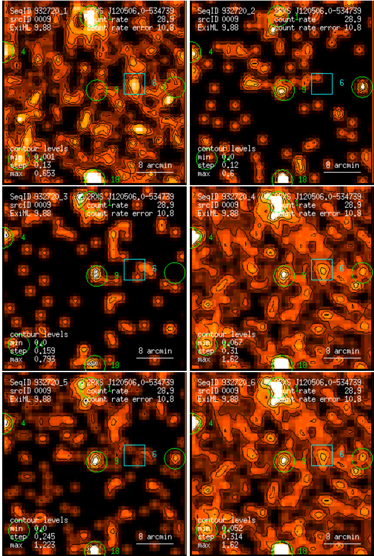
Figure 9: RASS 932720: detection 0009: band rate images, Gaussian filter: (1) PSPC channels 11 – 41, (2) 52 – 90, (3) 91 – 201, (4) 11 – 235, (5) 52 – 201, (6) 11 – 201. Broad band rates in counts/ks. Band rate contour levels in counts/ks/arcmin 2 .
