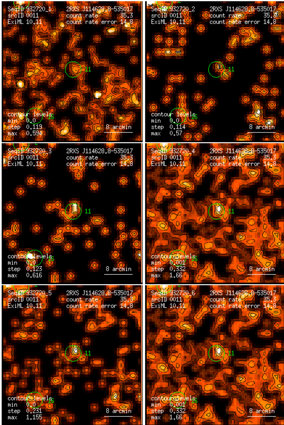
Figure 11: RASS 932720: detection 0011: band rate images, Gaussian filter: (1) PSPC channels 11 – 41, (2) 52 – 90, (3) 91 – 201, (4) 11 – 235, (5) 52 – 201, (6) 11 – 201. Broad band rates in counts/ks. Band rate contour levels in counts/ks/arcmin 2 .
