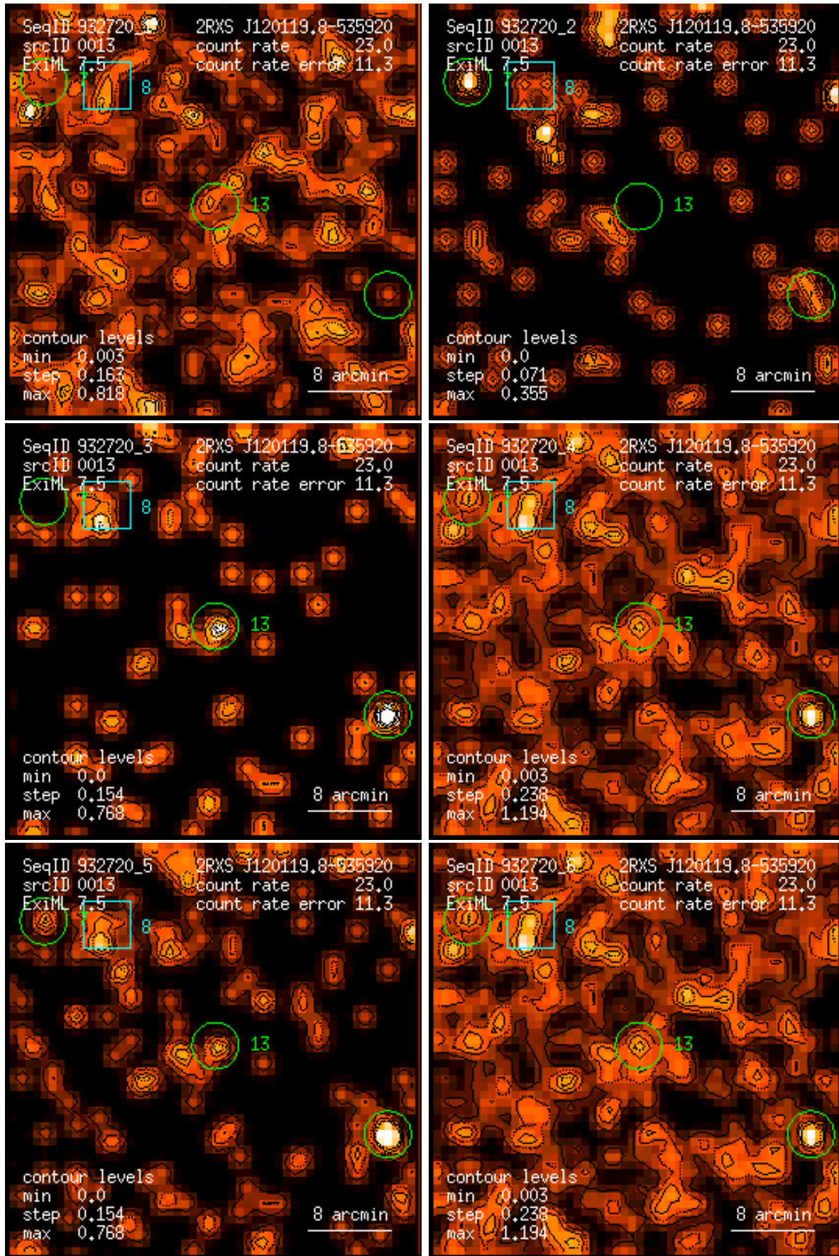
Figure 13: RASS 932720: detection 0013: band rate images, Gaussian filter: (1) PSPC channels 11 – 41, (2) 52 – 90, (3) 91 – 201, (4) 11 – 235, (5) 52 – 201, (6) 11 – 201. Broad band rates in counts/ks. Band rate contour levels in counts/ks/arcmin 2 .
