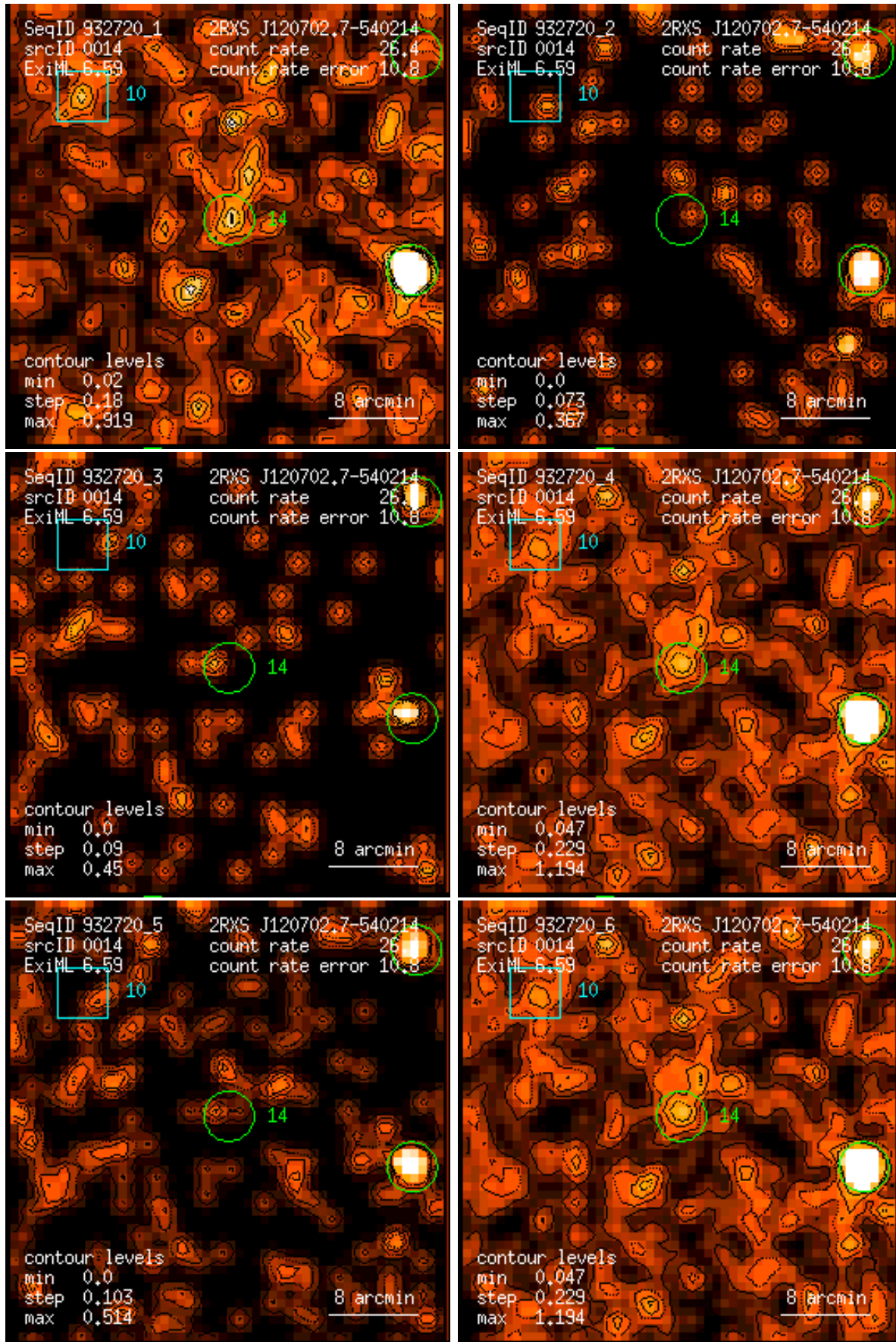
Figure 14: RASS 932720: detection 0014: band rate images, Gaussian filter: (1) PSPC channels 11 – 41, (2) 52 – 90, (3) 91 – 201, (4) 11 – 235, (5) 52 – 201, (6) 11 – 201. Broad band rates in counts/ks. Band rate contour levels in counts/ks/arcmin 2 .
