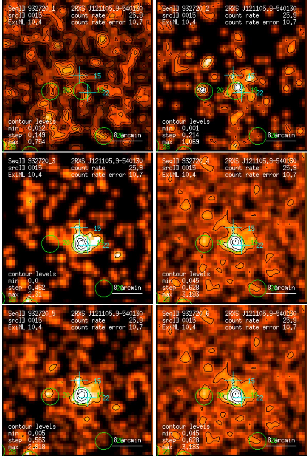
Figure 15: RASS 932720: detection 0015: band rate images, Gaussian filter: (1) PSPC channels 11 – 41, (2) 52 – 90, (3) 91 – 201, (4) 11 – 235, (5) 52 – 201, (6) 11 – 201. Broad band rates in counts/ks. Band rate contour levels in counts/ks/arcmin 2 .
