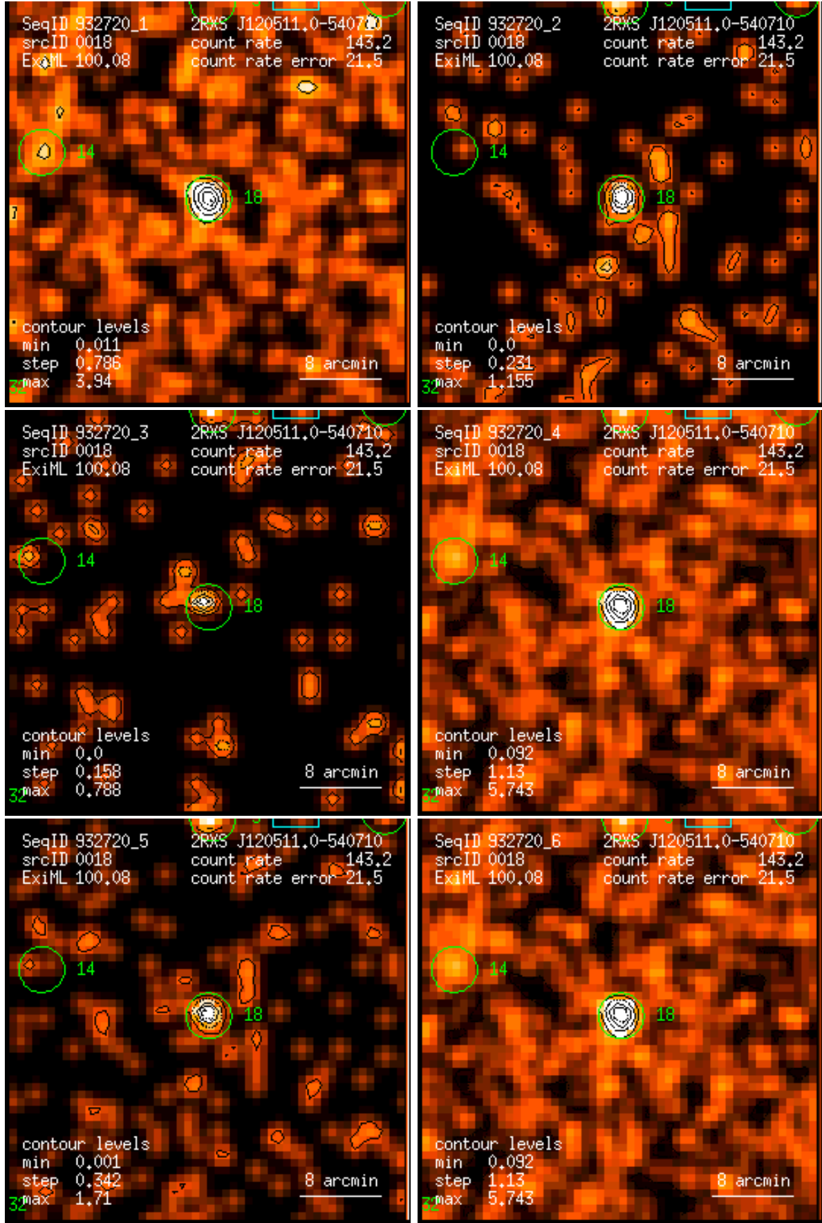
Figure 18: RASS 932720: detection 0018: band rate images, Gaussian filter: (1) PSPC channels 11 – 41, (2) 52 – 90, (3) 91 – 201, (4) 11 – 235, (5) 52 – 201, (6) 11 – 201. Broad band rates in counts/ks. Band rate contour levels in counts/ks/arcmin 2 .
