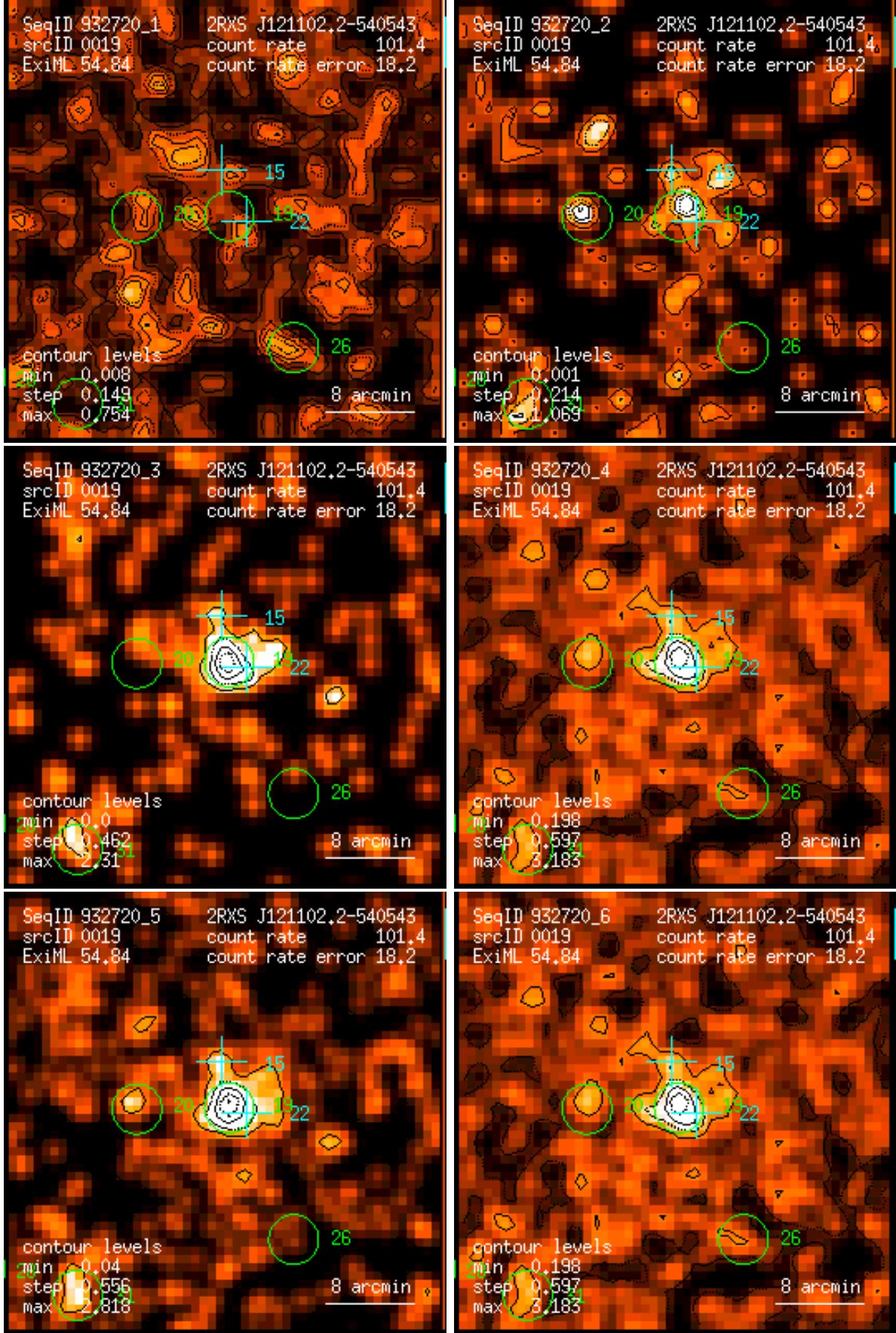
Figure 19: RASS 932720: detection 0019: band rate images, Gaussian filter: (1) PSPC channels 11 – 41, (2) 52 – 90, (3) 91 – 201, (4) 11 – 235, (5) 52 – 201, (6) 11 – 201. Broad band rates in counts/ks. Band rate contour levels in counts/ks/arcmin 2 .
