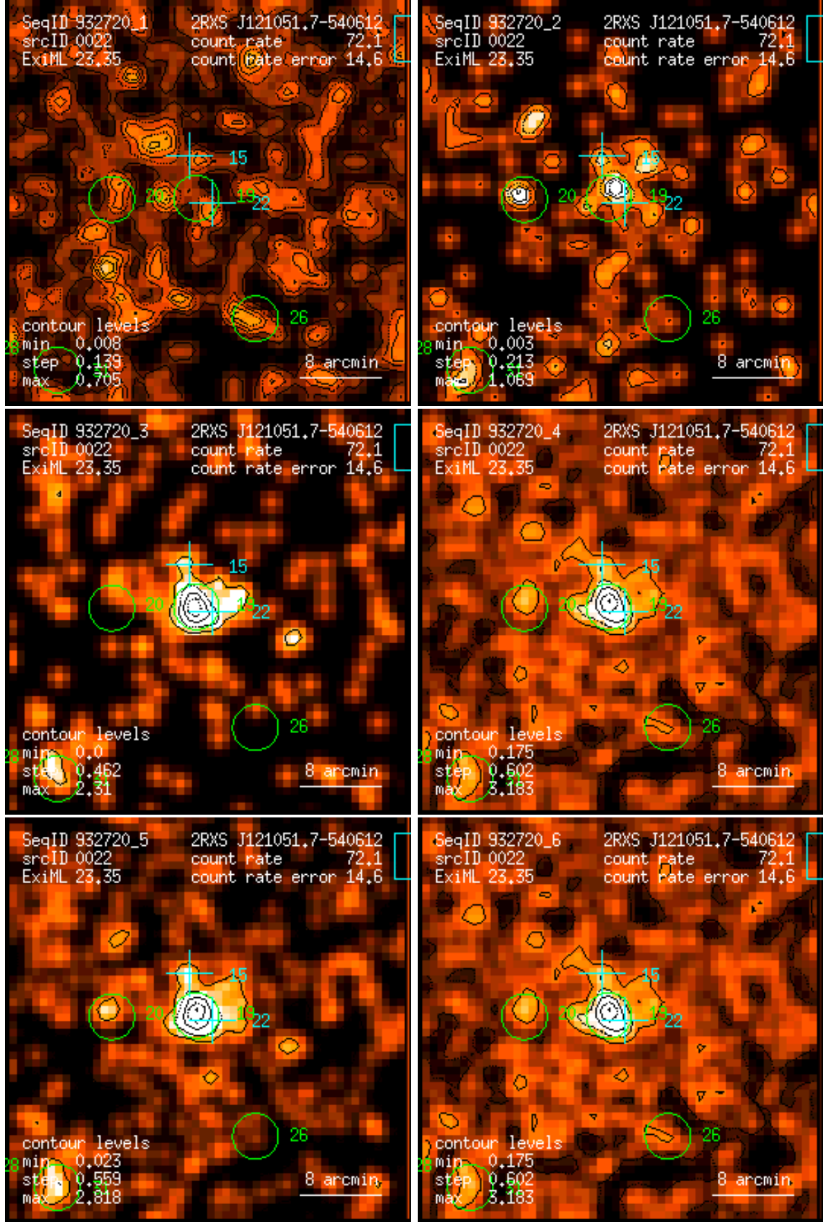
Figure 22: RASS 932720: detection 0022: band rate images, Gaussian filter: (1) PSPC channels 11 – 41, (2) 52 – 90, (3) 91 – 201, (4) 11 – 235, (5) 52 – 201, (6) 11 – 201. Broad band rates in counts/ks. Band rate contour levels in counts/ks/arcmin 2 .
