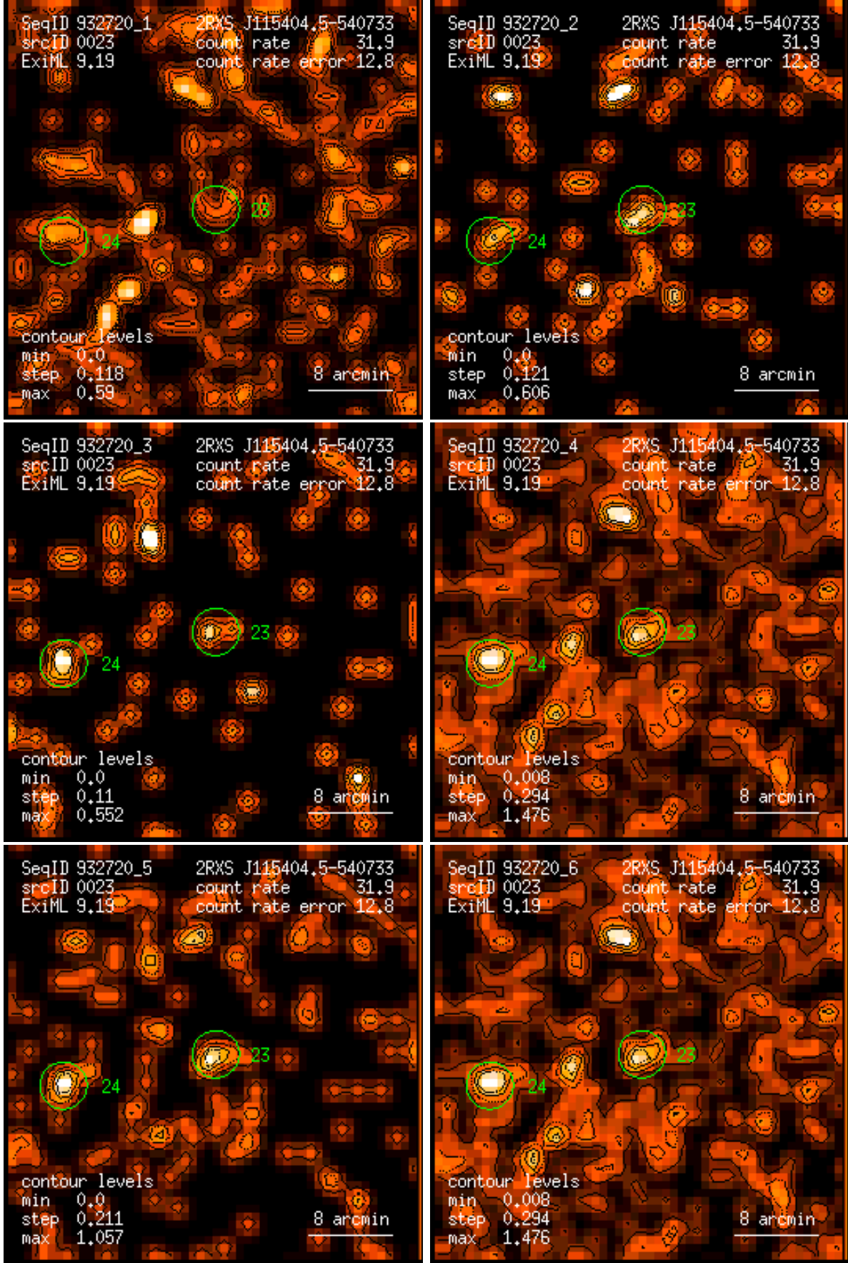
Figure 23: RASS 932720: detection 0023: band rate images, Gaussian filter: (1) PSPC channels 11 – 41, (2) 52 – 90, (3) 91 – 201, (4) 11 – 235, (5) 52 – 201, (6) 11 – 201. Broad band rates in counts/ks. Band rate contour levels in counts/ks/arcmin 2 .
