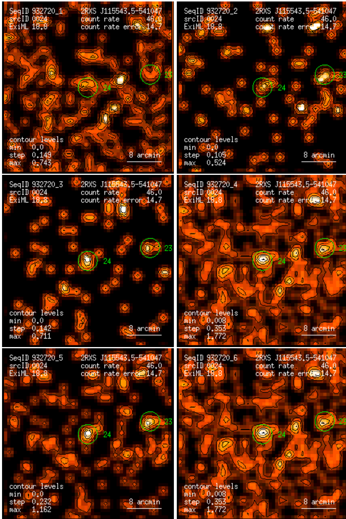
Figure 24: RASS 932720: detection 0024: band rate images, Gaussian filter: (1) PSPC channels 11 – 41, (2) 52 – 90, (3) 91 – 201, (4) 11 – 235, (5) 52 – 201, (6) 11 – 201. Broad band rates in counts/ks. Band rate contour levels in counts/ks/arcmin 2 .
