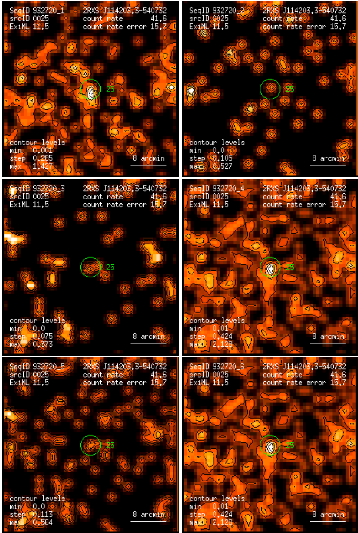
Figure 25: RASS 932720: detection 0025: band rate images, Gaussian filter: (1) PSPC channels 11 – 41, (2) 52 – 90, (3) 91 – 201, (4) 11 – 235, (5) 52 – 201, (6) 11 – 201. Broad band rates in counts/ks. Band rate contour levels in counts/ks/arcmin 2 .
