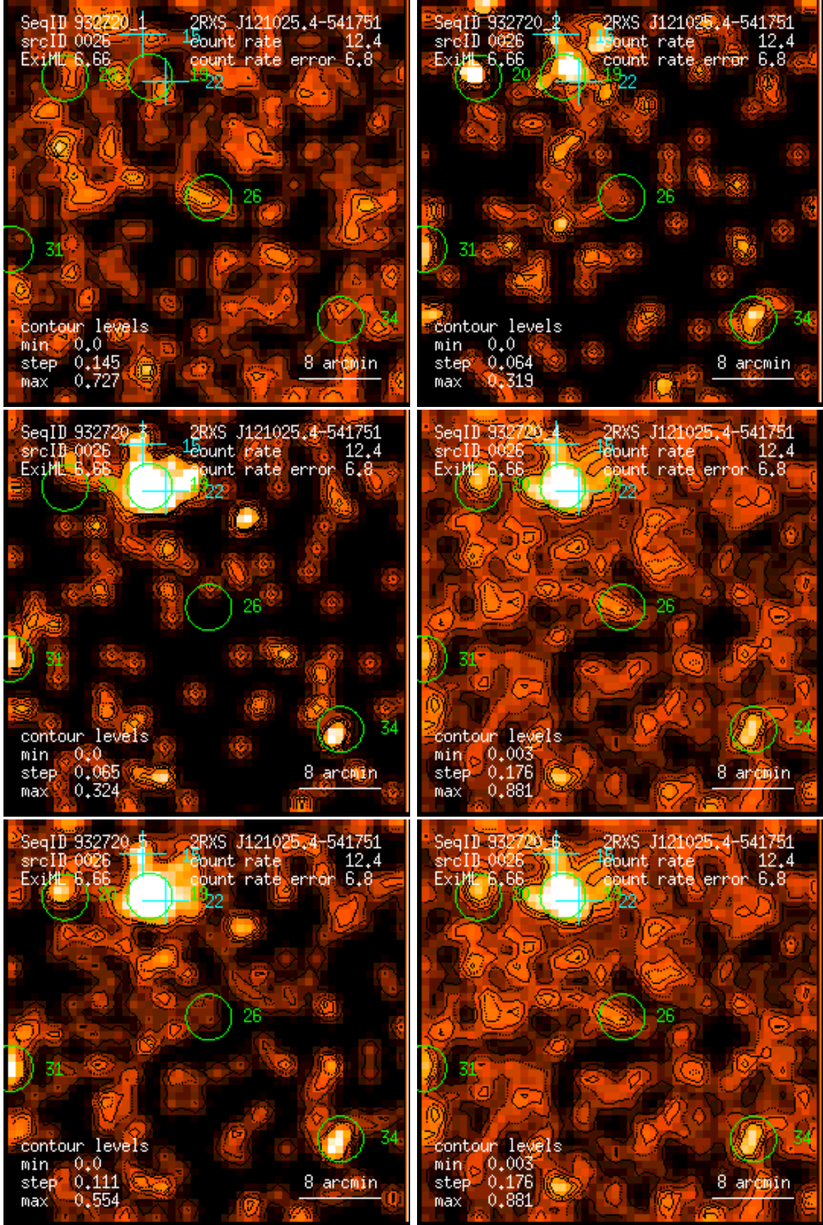
Figure 26: RASS 932720: detection 0026: band rate images, Gaussian filter: (1) PSPC channels 11 – 41, (2) 52 – 90, (3) 91 – 201, (4) 11 – 235, (5) 52 – 201, (6) 11 – 201. Broad band rates in counts/ks. Band rate contour levels in counts/ks/arcmin 2 .
