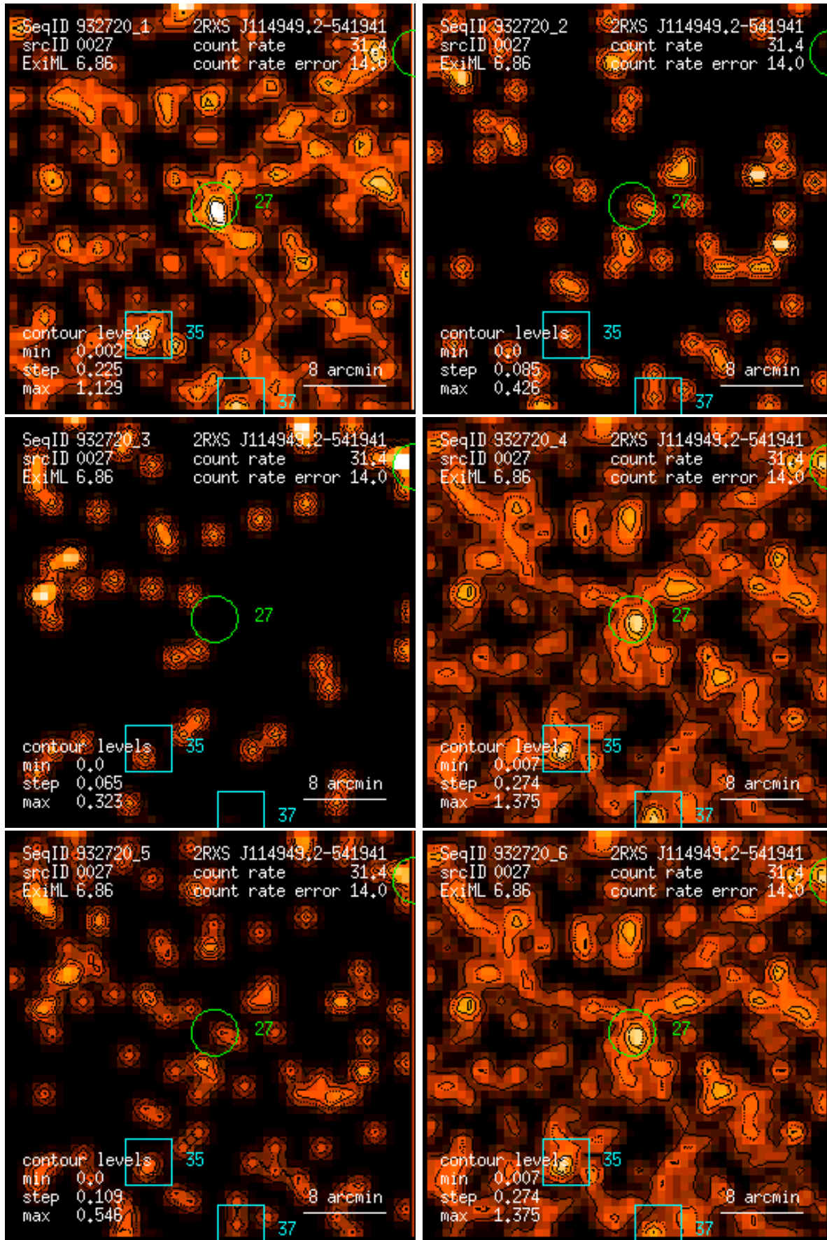
Figure 27: RASS 932720: detection 0027: band rate images, Gaussian filter: (1) PSPC channels 11 – 41, (2) 52 – 90, (3) 91 – 201, (4) 11 – 235, (5) 52 – 201, (6) 11 – 201. Broad band rates in counts/ks. Band rate contour levels in counts/ks/arcmin 2 .
