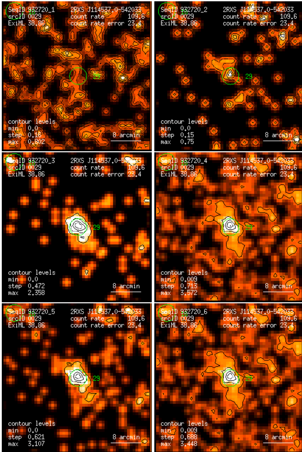
Figure 29: RASS 932720: detection 0029: band rate images, Gaussian filter: (1) PSPC channels 11 – 41, (2) 52 – 90, (3) 91 – 201, (4) 11 – 235, (5) 52 – 201, (6) 11 – 201. Broad band rates in counts/ks. Band rate contour levels in counts/ks/arcmin 2 .
