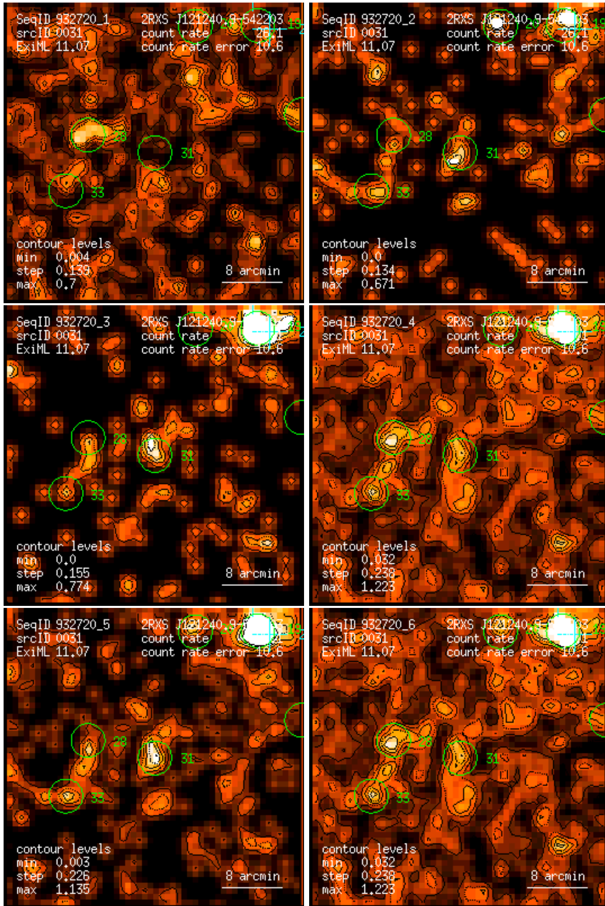
Figure 31: RASS 932720: detection 0031: band rate images, Gaussian filter: (1) PSPC channels 11 – 41, (2) 52 – 90, (3) 91 – 201, (4) 11 – 235, (5) 52 – 201, (6) 11 – 201. Broad band rates in counts/ks. Band rate contour levels in counts/ks/arcmin 2 .
