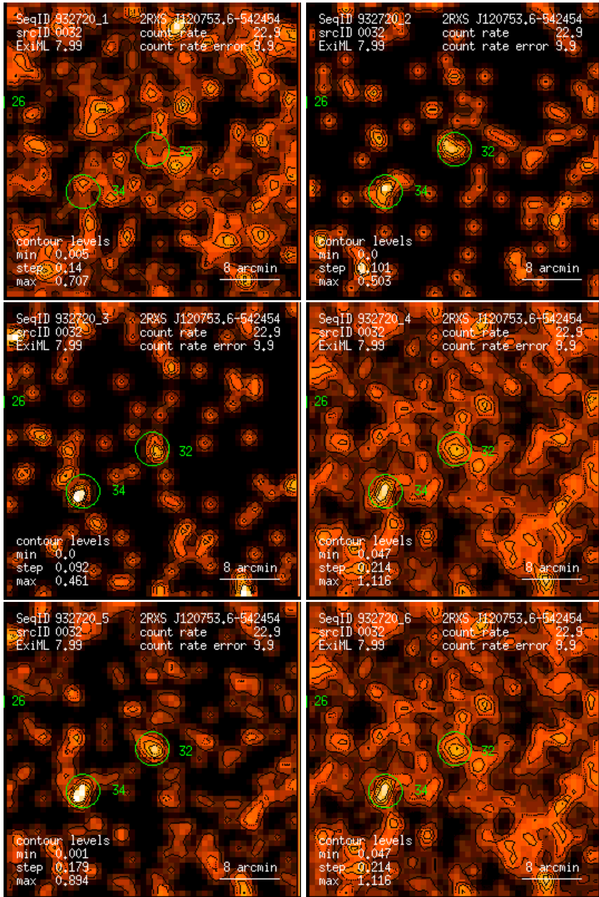
Figure 32: RASS 932720: detection 0032: band rate images, Gaussian filter: (1) PSPC channels 11 – 41, (2) 52 – 90, (3) 91 – 201, (4) 11 – 235, (5) 52 – 201, (6) 11 – 201. Broad band rates in counts/ks. Band rate contour levels in counts/ks/arcmin 2 .
