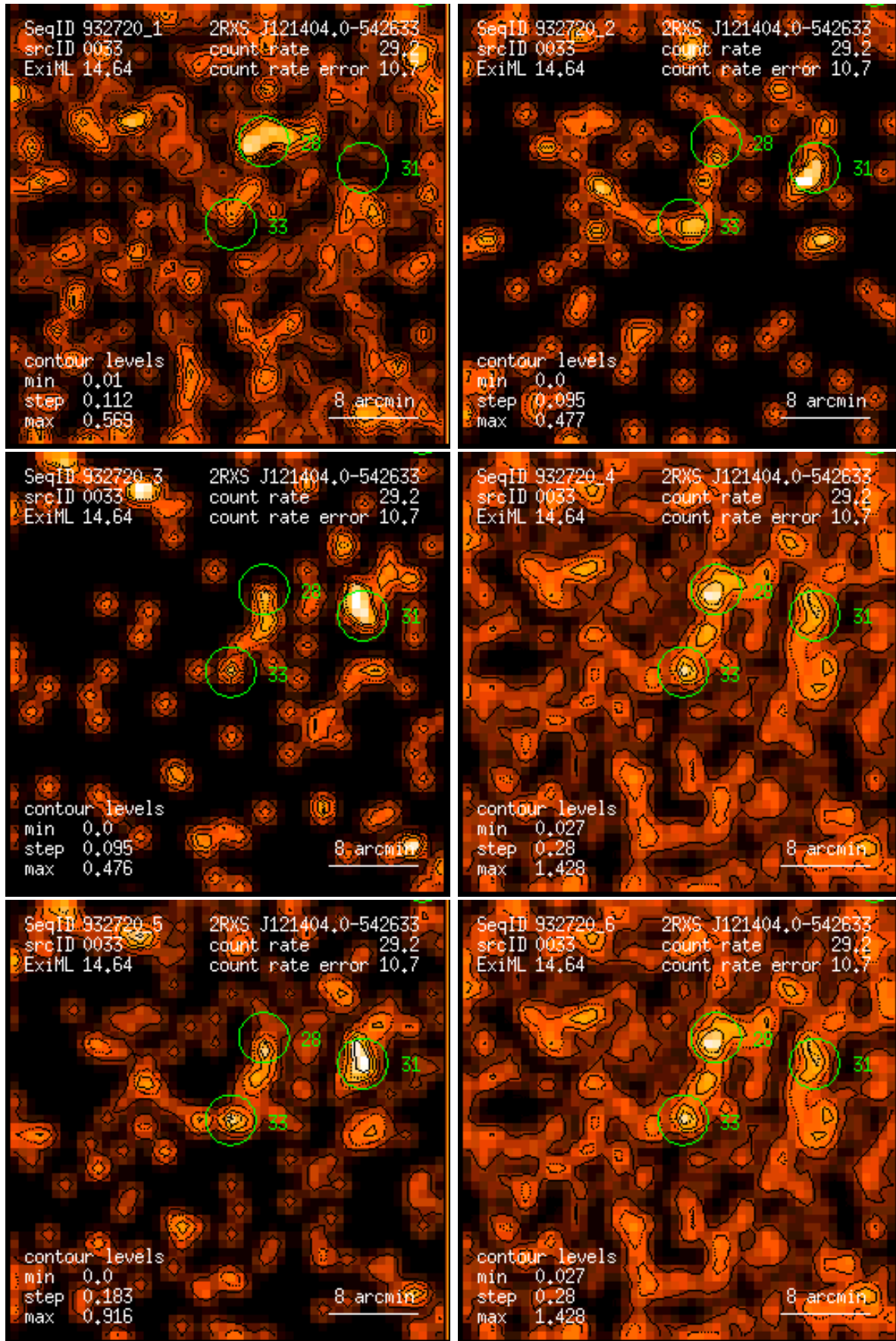
Figure 33: RASS 932720: detection 0033: band rate images, Gaussian filter: (1) PSPC channels 11 – 41, (2) 52 – 90, (3) 91 – 201, (4) 11 – 235, (5) 52 – 201, (6) 11 – 201. Broad band rates in counts/ks. Band rate contour levels in counts/ks/arcmin 2 .
