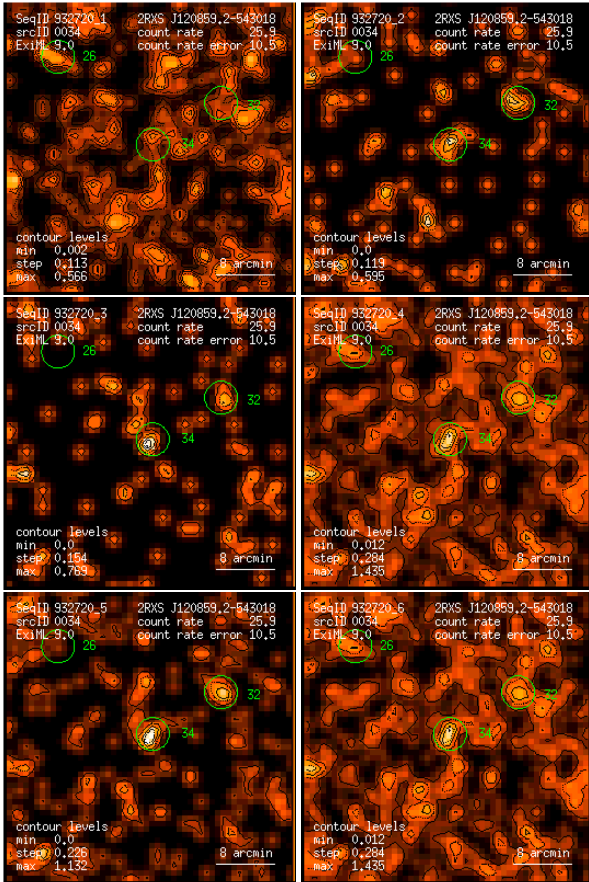
Figure 34: RASS 932720: detection 0034: band rate images, Gaussian filter: (1) PSPC channels 11 – 41, (2) 52 – 90, (3) 91 – 201, (4) 11 – 235, (5) 52 – 201, (6) 11 – 201. Broad band rates in counts/ks. Band rate contour levels in counts/ks/arcmin 2 .
