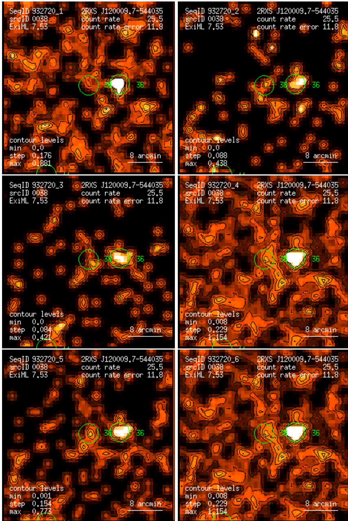
Figure 38: RASS 932720: detection 0038: band rate images, Gaussian filter: (1) PSPC channels 11 – 41, (2) 52 – 90, (3) 91 – 201, (4) 11 – 235, (5) 52 – 201, (6) 11 – 201. Broad band rates in counts/ks. Band rate contour levels in counts/ks/arcmin 2 .
