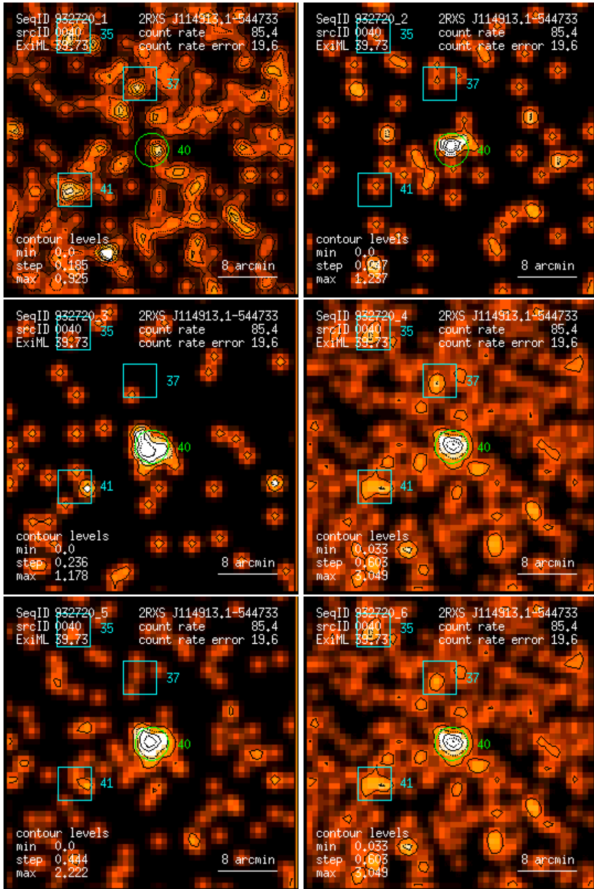
Figure 40: RASS 932720: detection 0040: band rate images, Gaussian filter: (1) PSPC channels 11 – 41, (2) 52 – 90, (3) 91 – 201, (4) 11 – 235, (5) 52 – 201, (6) 11 – 201. Broad band rates in counts/ks. Band rate contour levels in counts/ks/arcmin 2 .
