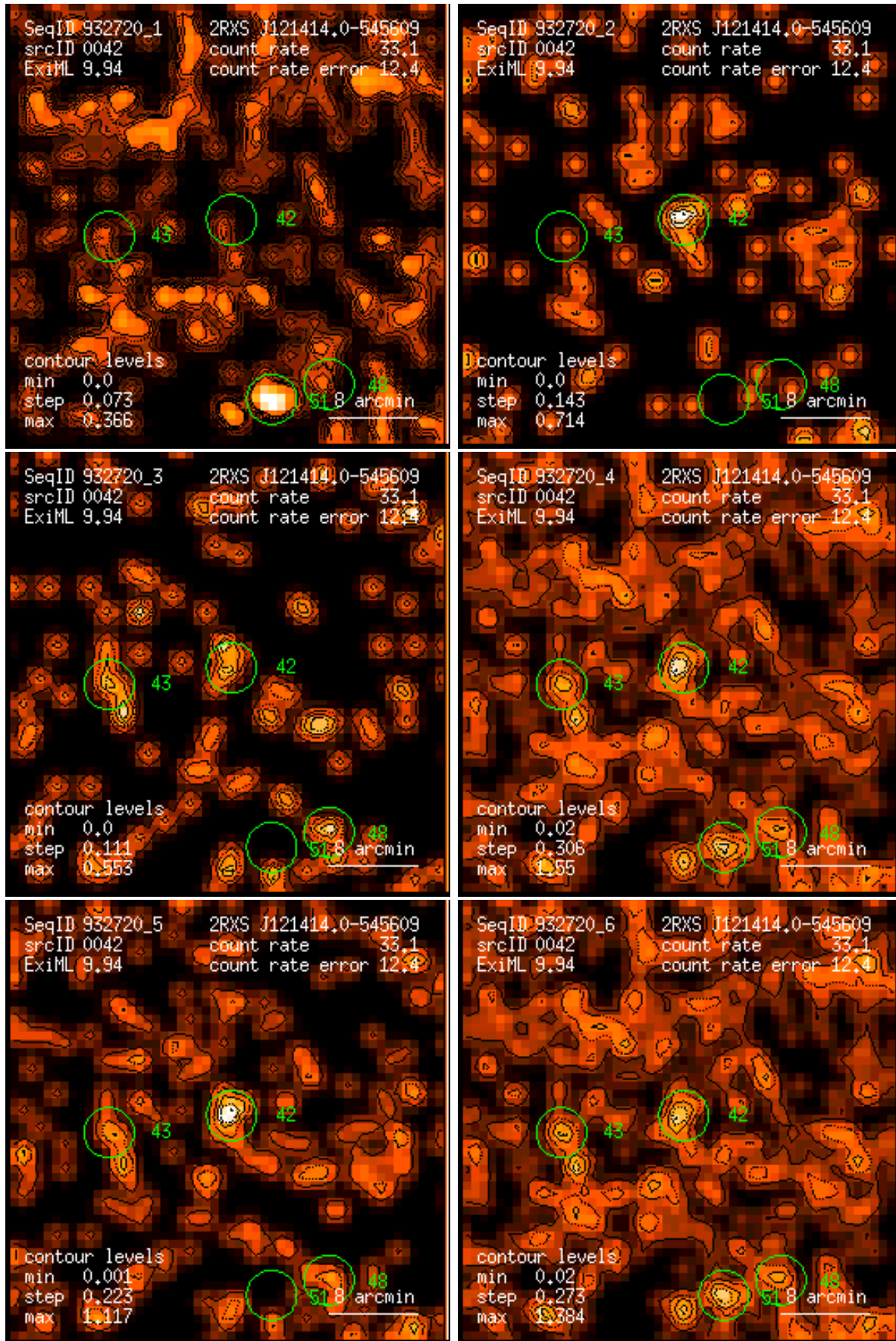
Figure 42: RASS 932720: detection 0042: band rate images, Gaussian filter: (1) PSPC channels 11 – 41, (2) 52 – 90, (3) 91 – 201, (4) 11 – 235, (5) 52 – 201, (6) 11 – 201. Broad band rates in counts/ks. Band rate contour levels in counts/ks/arcmin 2 .
