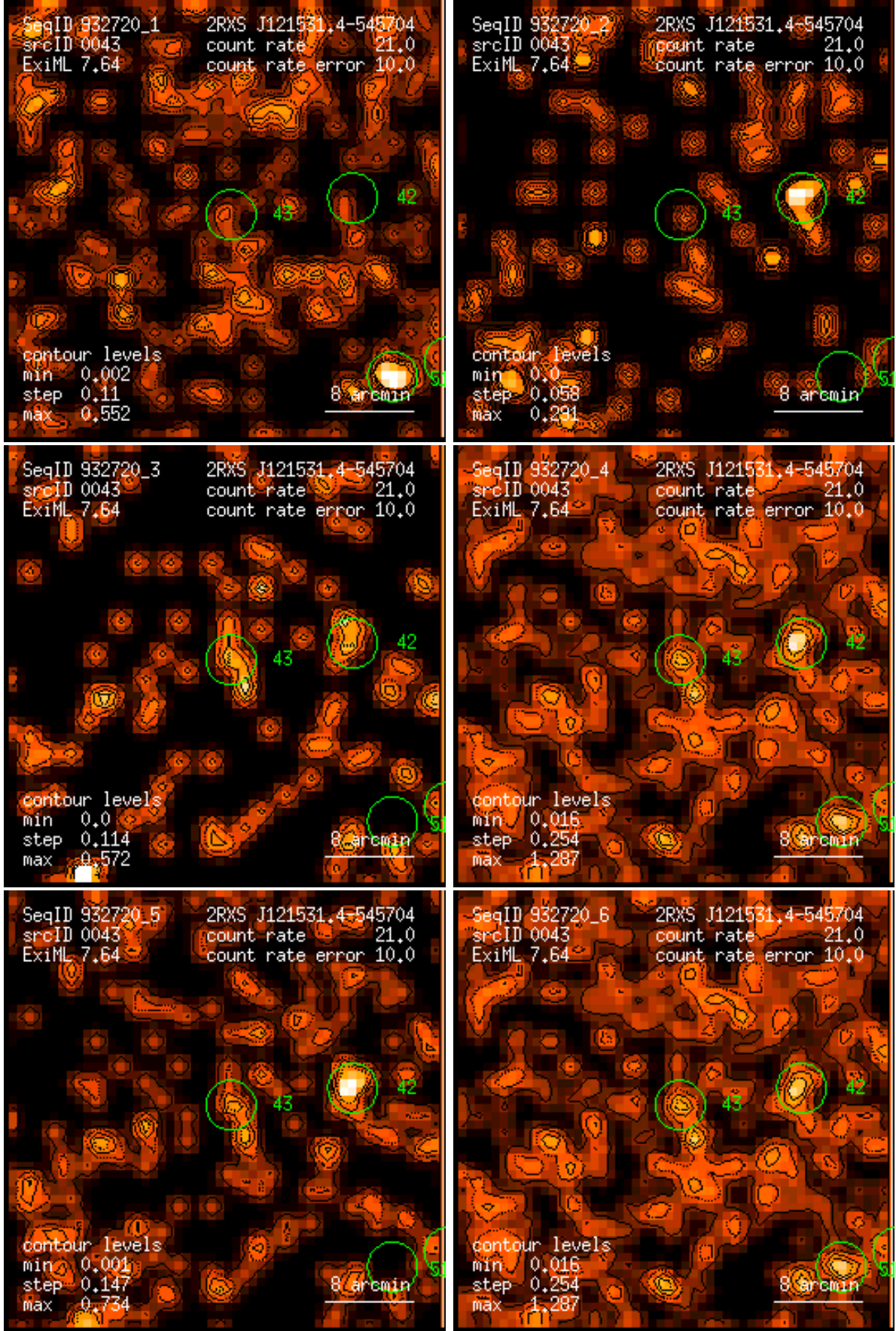
Figure 43: RASS 932720: detection 0043: band rate images, Gaussian filter: (1) PSPC channels 11 – 41, (2) 52 – 90, (3) 91 – 201, (4) 11 – 235, (5) 52 – 201, (6) 11 – 201. Broad band rates in counts/ks. Band rate contour levels in counts/ks/arcmin 2 .
