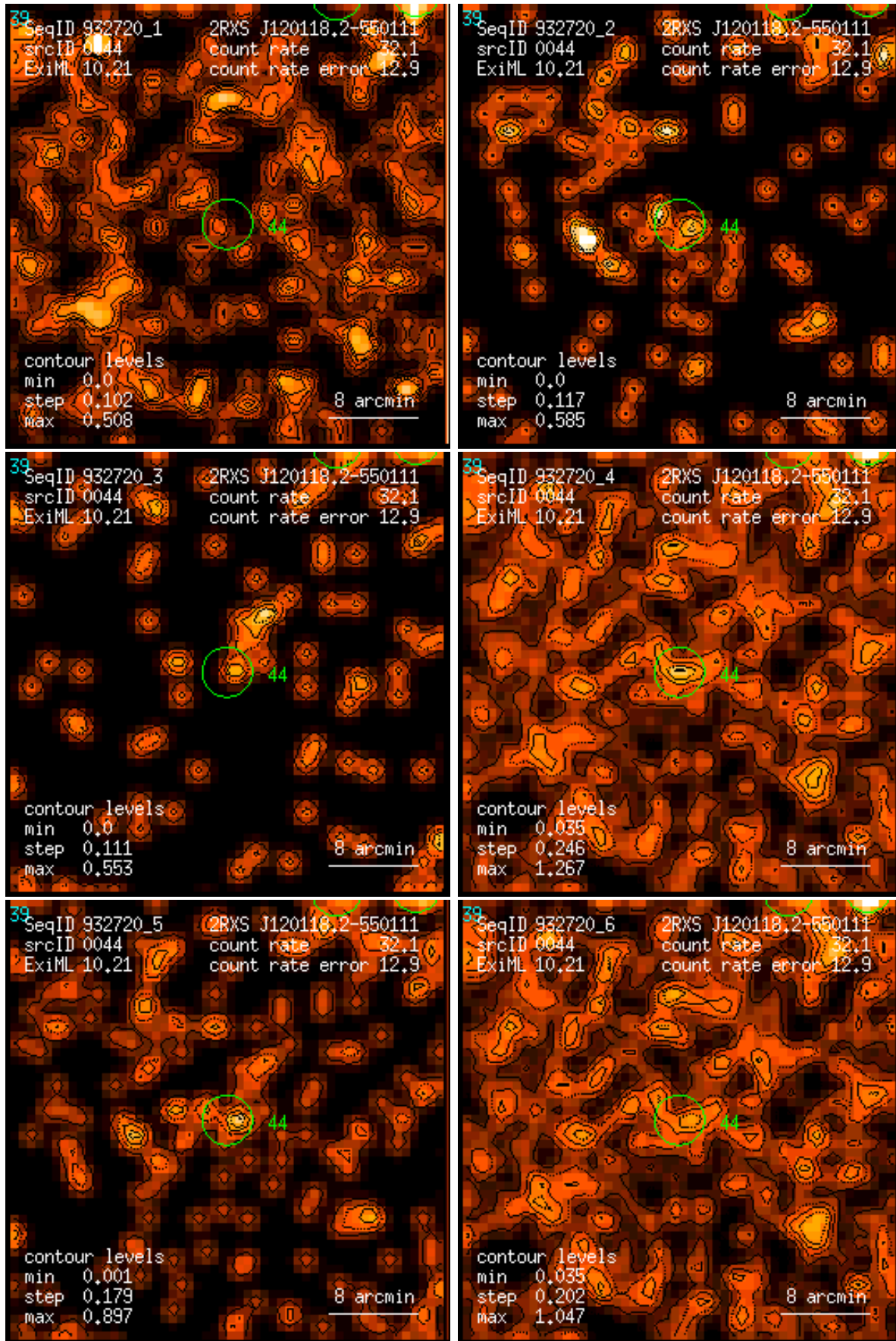
Figure 44: RASS 932720: detection 0044: band rate images, Gaussian filter: (1) PSPC channels 11 – 41, (2) 52 – 90, (3) 91 – 201, (4) 11 – 235, (5) 52 – 201, (6) 11 – 201. Broad band rates in counts/ks. Band rate contour levels in counts/ks/arcmin 2 .
