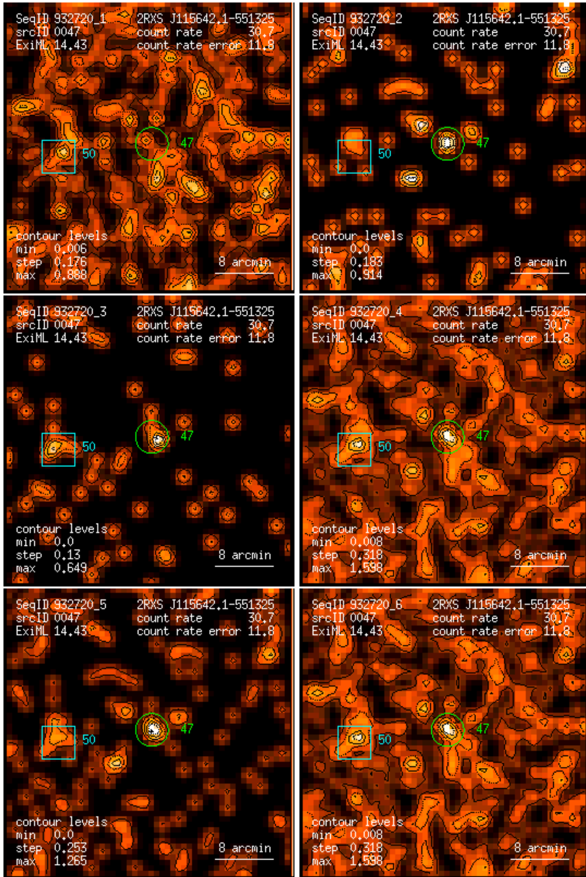
Figure 47: RASS 932720: detection 0047: band rate images, Gaussian filter: (1) PSPC channels 11 – 41, (2) 52 – 90, (3) 91 – 201, (4) 11 – 235, (5) 52 – 201, (6) 11 – 201. Broad band rates in counts/ks. Band rate contour levels in counts/ks/arcmin 2 .
