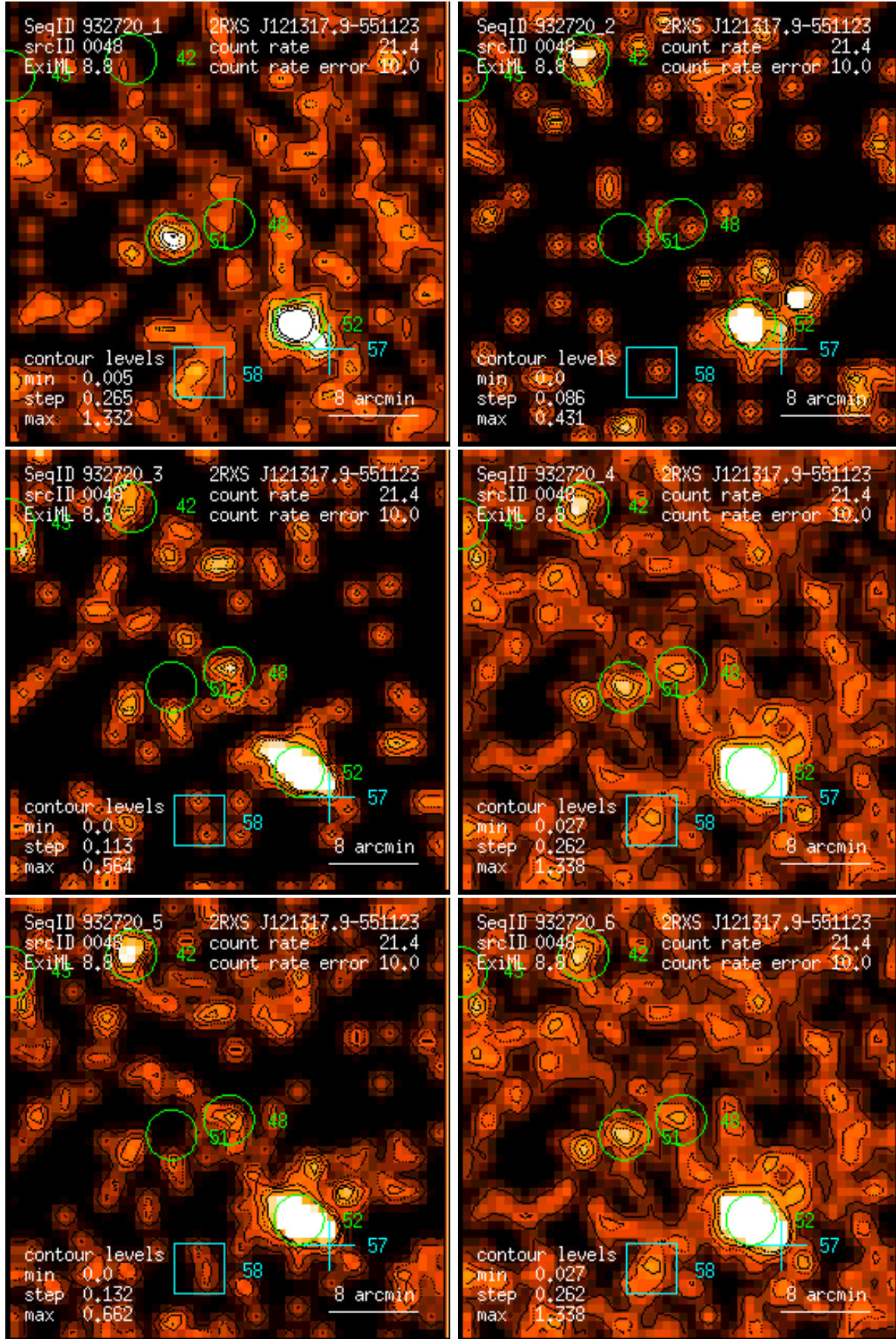
Figure 48: RASS 932720: detection 0048: band rate images, Gaussian filter: (1) PSPC channels 11 – 41, (2) 52 – 90, (3) 91 – 201, (4) 11 – 235, (5) 52 – 201, (6) 11 – 201. Broad band rates in counts/ks. Band rate contour levels in counts/ks/arcmin 2 .
