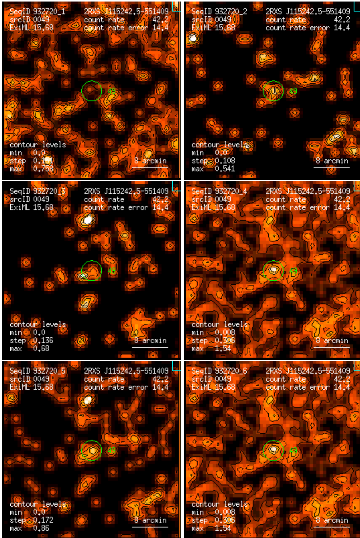
Figure 49: RASS 932720: detection 0049: band rate images, Gaussian filter: (1) PSPC channels 11 – 41, (2) 52 – 90, (3) 91 – 201, (4) 11 – 235, (5) 52 – 201, (6) 11 – 201. Broad band rates in counts/ks. Band rate contour levels in counts/ks/arcmin 2 .
