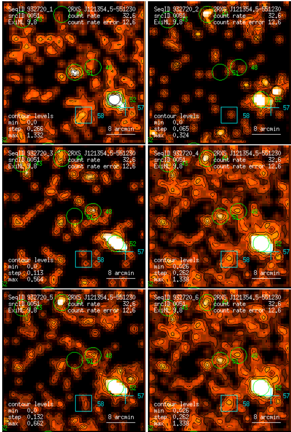
Figure 51: RASS 932720: detection 0051: band rate images, Gaussian filter: (1) PSPC channels 11 – 41, (2) 52 – 90, (3) 91 – 201, (4) 11 – 235, (5) 52 – 201, (6) 11 – 201. Broad band rates in counts/ks. Band rate contour levels in counts/ks/arcmin 2 .
