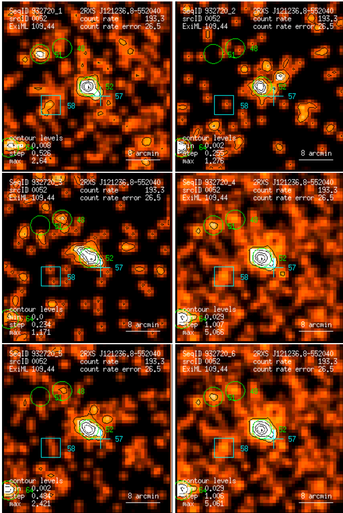
Figure 52: RASS 932720: detection 0052: band rate images, Gaussian filter: (1) PSPC channels 11 – 41, (2) 52 – 90, (3) 91 – 201, (4) 11 – 235, (5) 52 – 201, (6) 11 – 201. Broad band rates in counts/ks. Band rate contour levels in counts/ks/arcmin 2 .
