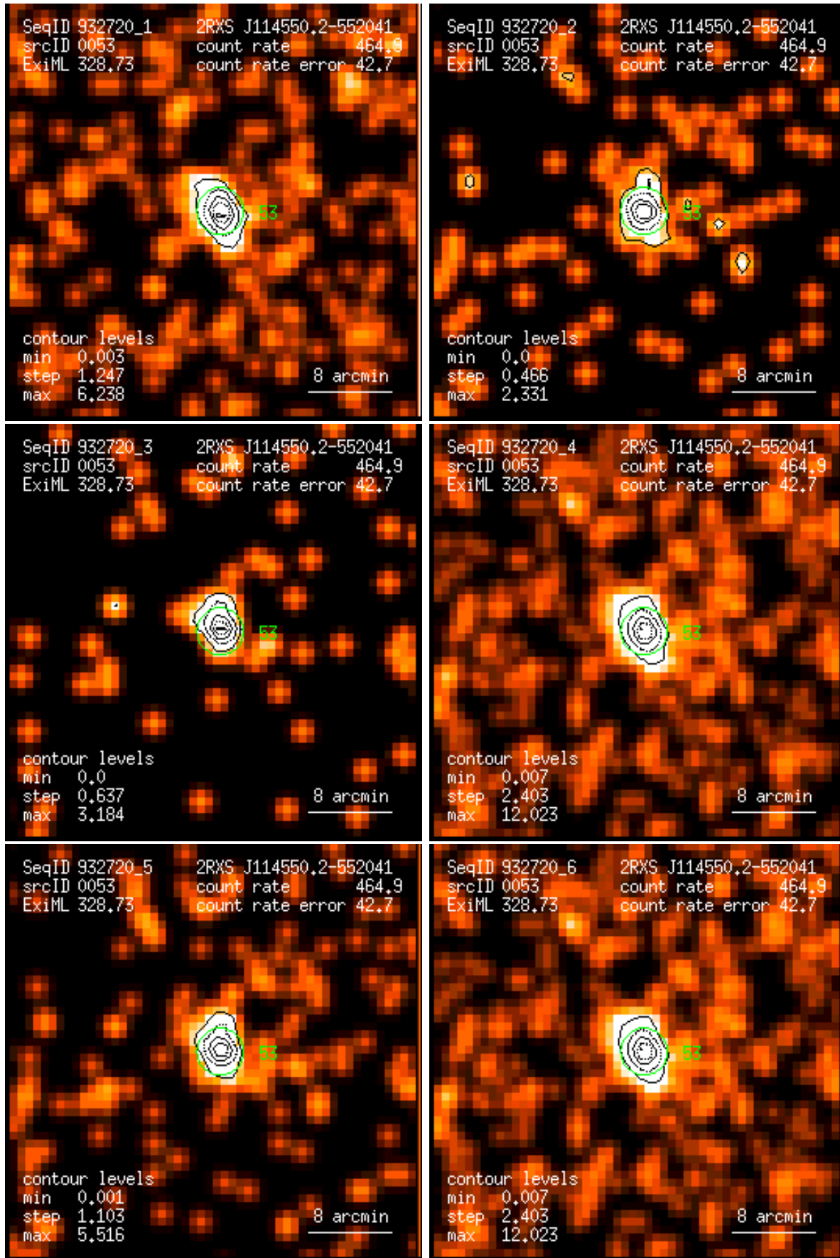
Figure 53: RASS 932720: detection 0053: band rate images, Gaussian filter: (1) PSPC channels 11 – 41, (2) 52 – 90, (3) 91 – 201, (4) 11 – 235, (5) 52 – 201, (6) 11 – 201. Broad band rates in counts/ks. Band rate contour levels in counts/ks/arcmin 2 .
