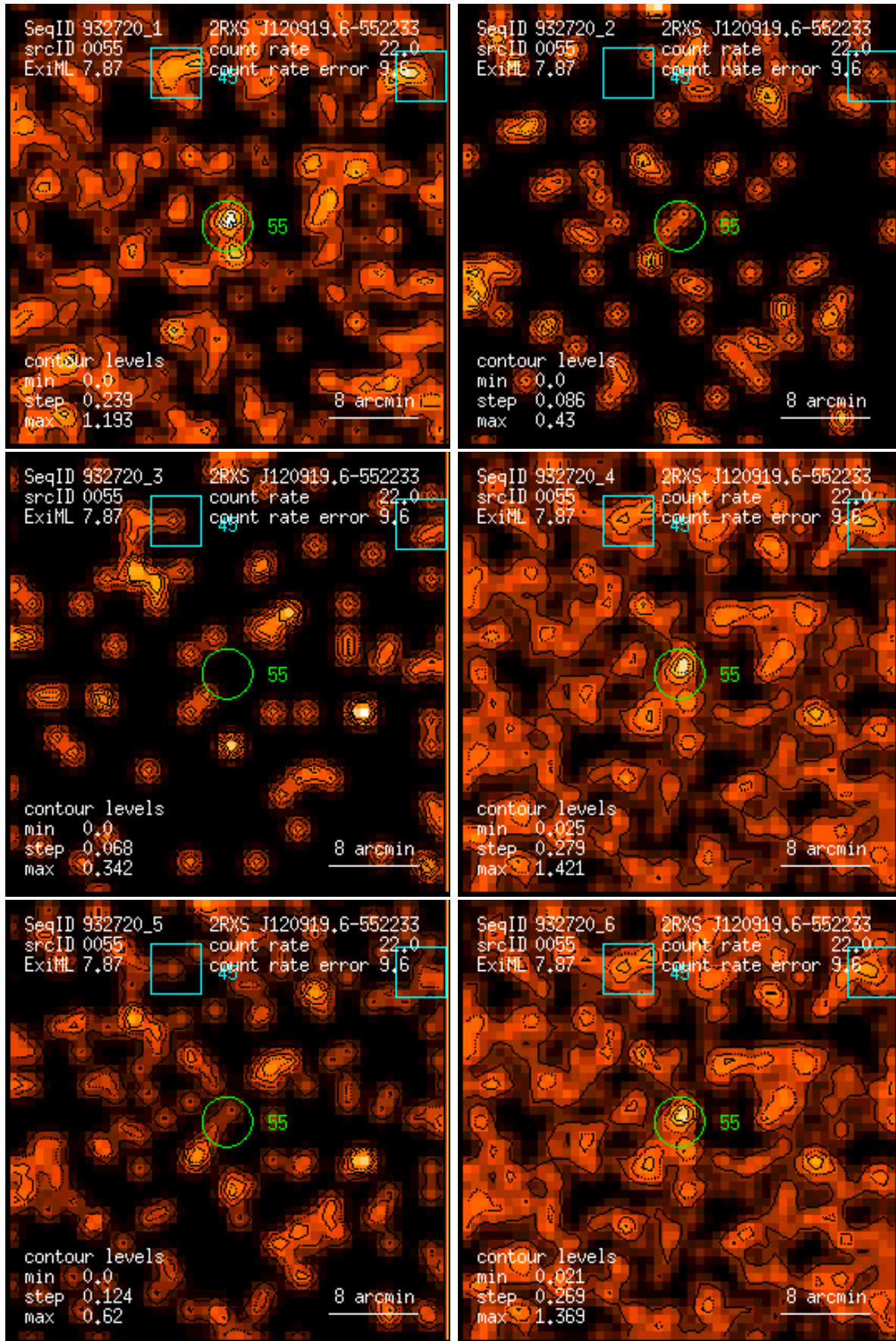
Figure 55: RASS 932720: detection 0055: band rate images, Gaussian filter: (1) PSPC channels 11 – 41, (2) 52 – 90, (3) 91 – 201, (4) 11 – 235, (5) 52 – 201, (6) 11 – 201. Broad band rates in counts/ks. Band rate contour levels in counts/ks/arcmin 2 .
