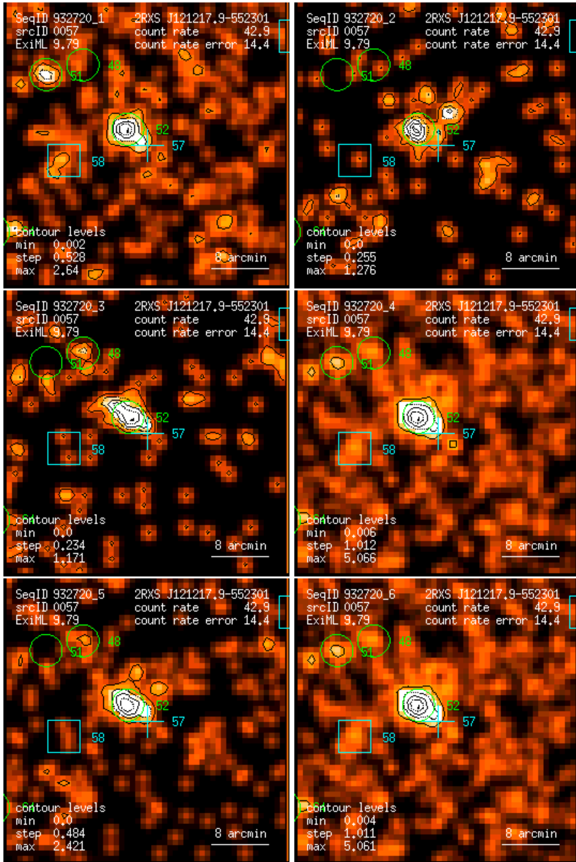
Figure 57: RASS 932720: detection 0057: band rate images, Gaussian filter: (1) PSPC channels 11 – 41, (2) 52 – 90, (3) 91 – 201, (4) 11 – 235, (5) 52 – 201, (6) 11 – 201. Broad band rates in counts/ks. Band rate contour levels in counts/ks/arcmin 2 .
