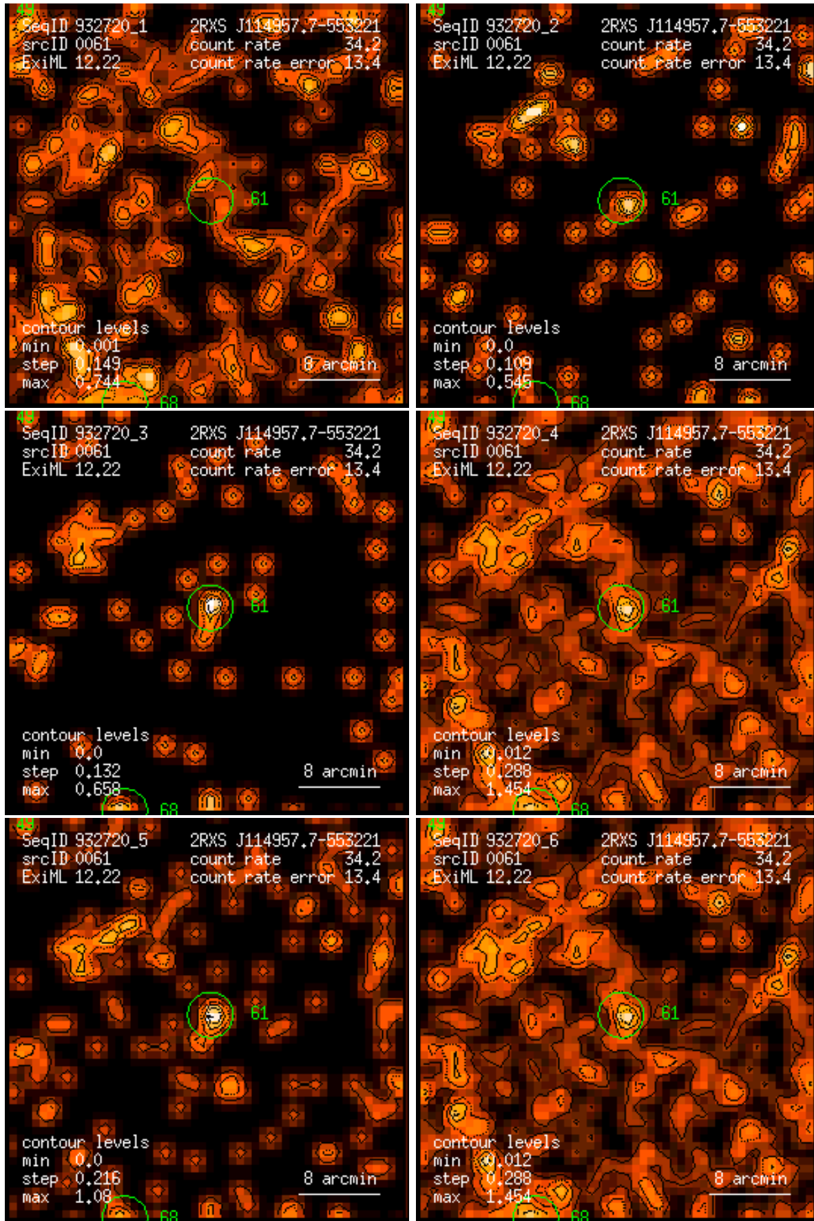
Figure 61: RASS 932720: detection 0061: band rate images, Gaussian filter: (1) PSPC channels 11 – 41, (2) 52 – 90, (3) 91 – 201, (4) 11 – 235, (5) 52 – 201, (6) 11 – 201. Broad band rates in counts/ks. Band rate contour levels in counts/ks/arcmin 2 .
