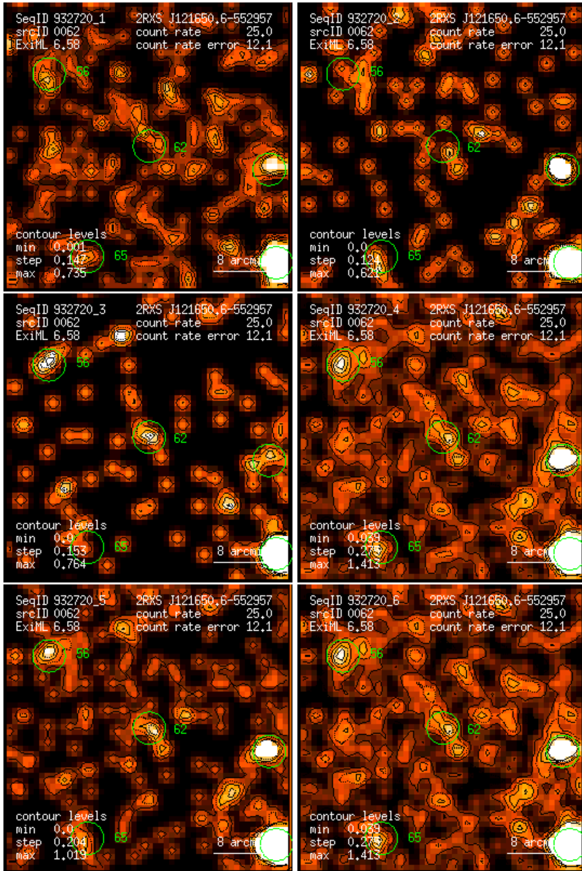
Figure 62: RASS 932720: detection 0062: band rate images, Gaussian filter: (1) PSPC channels 11 – 41, (2) 52 – 90, (3) 91 – 201, (4) 11 – 235, (5) 52 – 201, (6) 11 – 201. Broad band rates in counts/ks. Band rate contour levels in counts/ks/arcmin 2 .
