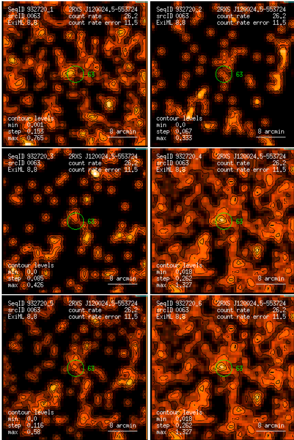
Figure 63: RASS 932720: detection 0063: band rate images, Gaussian filter: (1) PSPC channels 11 – 41, (2) 52 – 90, (3) 91 – 201, (4) 11 – 235, (5) 52 – 201, (6) 11 – 201. Broad band rates in counts/ks. Band rate contour levels in counts/ks/arcmin 2 .
