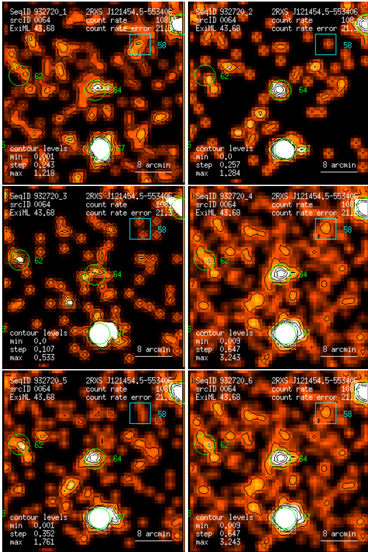
Figure 64: RASS 932720: detection 0064: band rate images, Gaussian filter: (1) PSPC channels 11 – 41, (2) 52 – 90, (3) 91 – 201, (4) 11 – 235, (5) 52 – 201, (6) 11 – 201. Broad band rates in counts/ks. Band rate contour levels in counts/ks/arcmin 2 .
