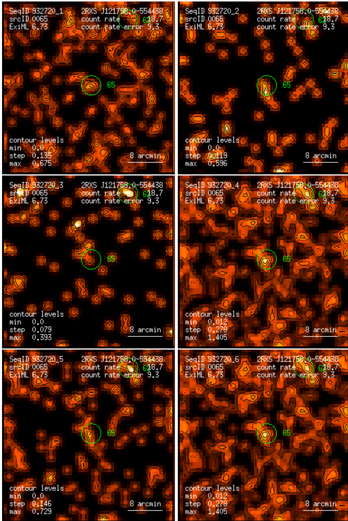
Figure 65: RASS 932720: detection 0065: band rate images, Gaussian filter: (1) PSPC channels 11 – 41, (2) 52 – 90, (3) 91 – 201, (4) 11 – 235, (5) 52 – 201, (6) 11 – 201. Broad band rates in counts/ks. Band rate contour levels in counts/ks/arcmin 2 .
