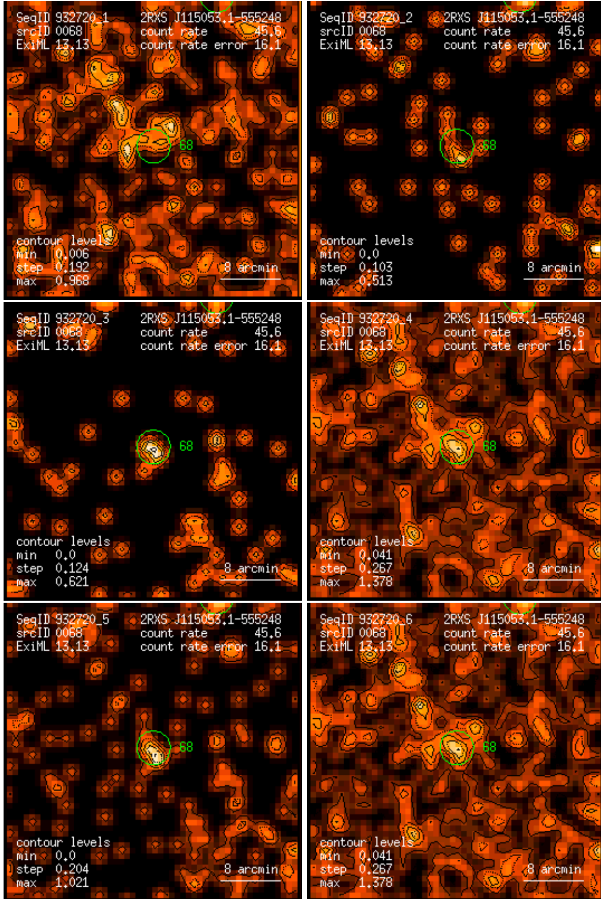
Figure 68: RASS 932720: detection 0068: band rate images, Gaussian filter: (1) PSPC channels 11 – 41, (2) 52 – 90, (3) 91 – 201, (4) 11 – 235, (5) 52 – 201, (6) 11 – 201. Broad band rates in counts/ks. Band rate contour levels in counts/ks/arcmin 2 .
