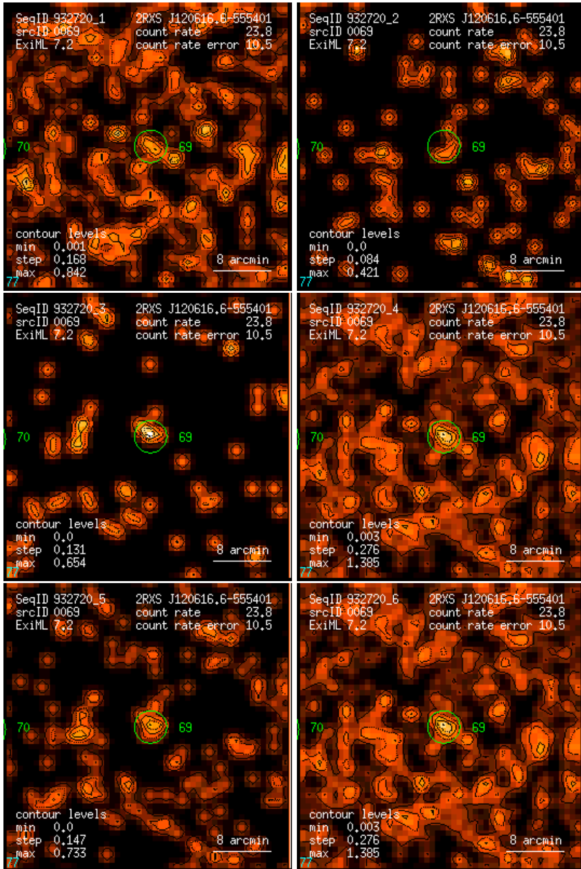
Figure 69: RASS 932720: detection 0069: band rate images, Gaussian filter: (1) PSPC channels 11 – 41, (2) 52 – 90, (3) 91 – 201, (4) 11 – 235, (5) 52 – 201, (6) 11 – 201. Broad band rates in counts/ks. Band rate contour levels in counts/ks/arcmin 2 .
