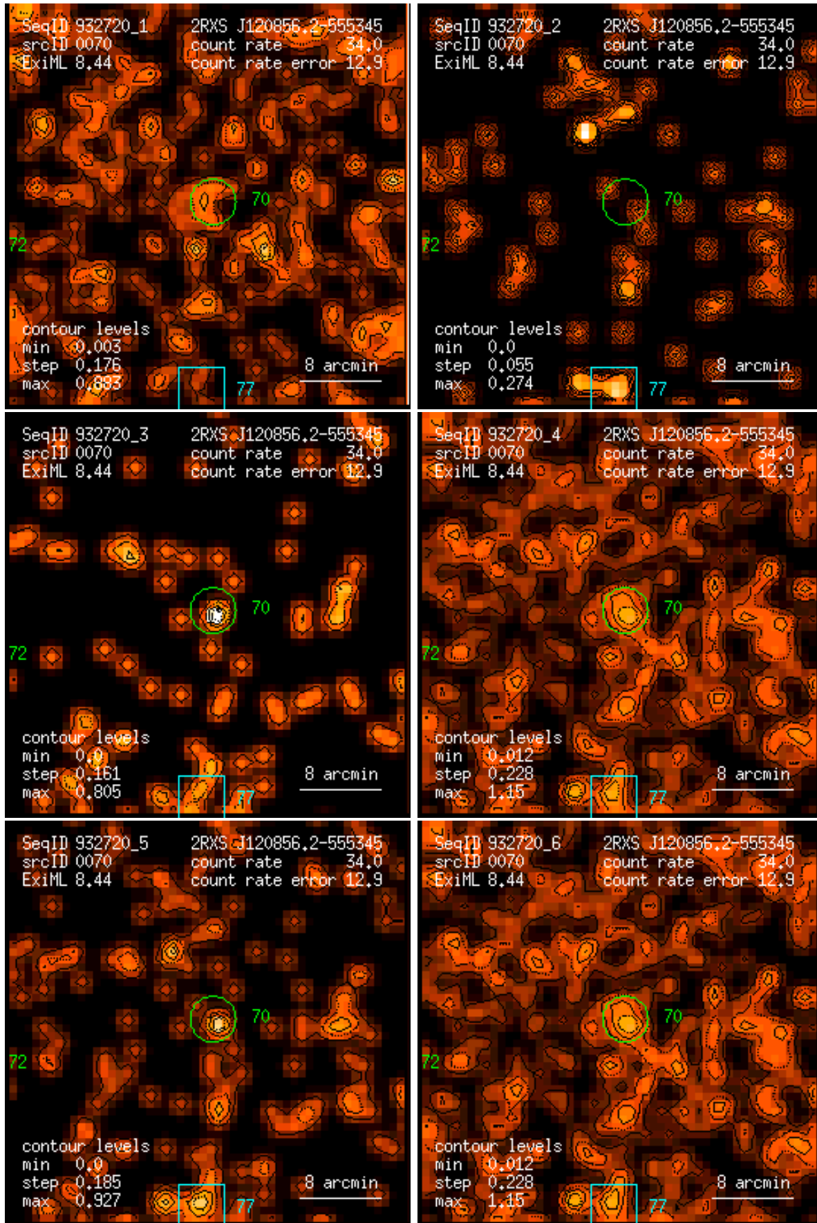
Figure 70: RASS 932720: detection 0070: band rate images, Gaussian filter: (1) PSPC channels 11 – 41, (2) 52 – 90, (3) 91 – 201, (4) 11 – 235, (5) 52 – 201, (6) 11 – 201. Broad band rates in counts/ks. Band rate contour levels in counts/ks/arcmin 2 .
