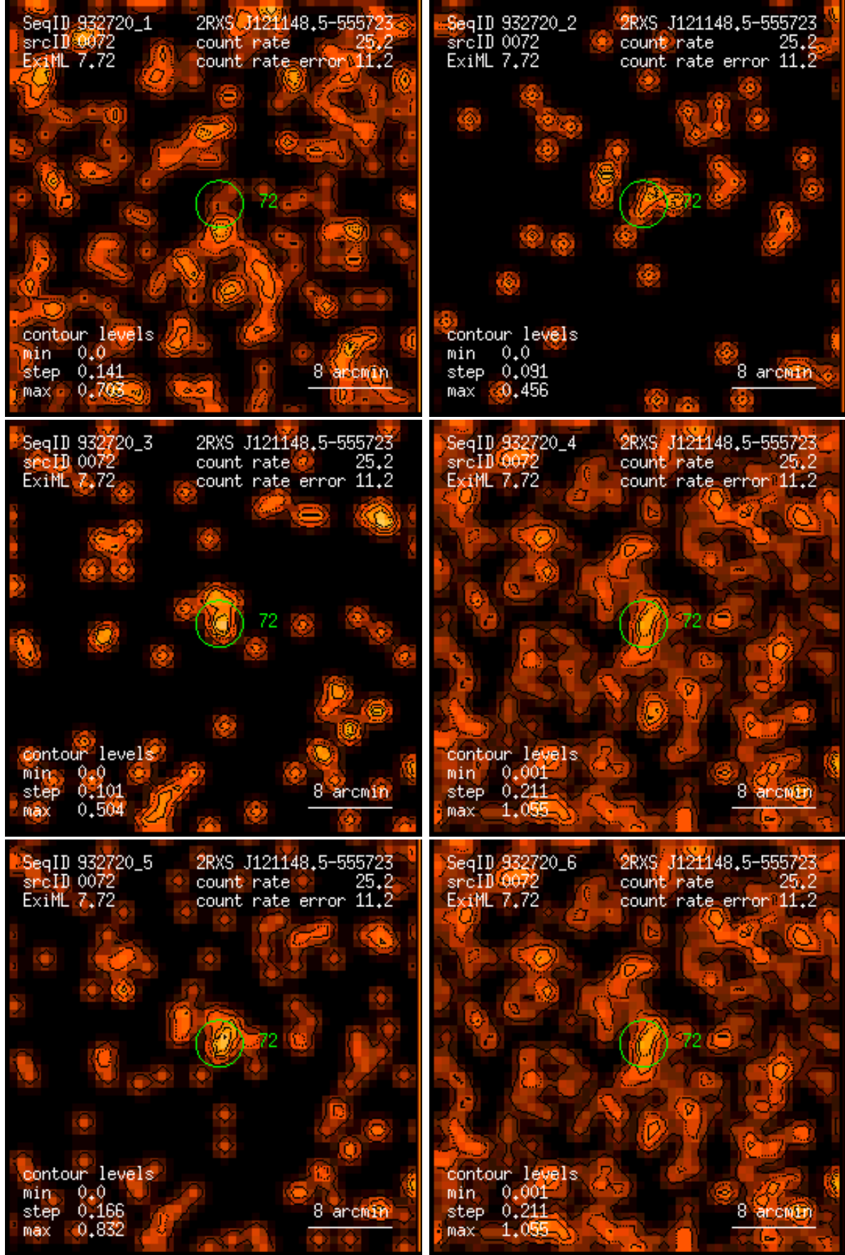
Figure 72: RASS 932720: detection 0072: band rate images, Gaussian filter: (1) PSPC channels 11 – 41, (2) 52 – 90, (3) 91 – 201, (4) 11 – 235, (5) 52 – 201, (6) 11 – 201. Broad band rates in counts/ks. Band rate contour levels in counts/ks/arcmin 2 .
