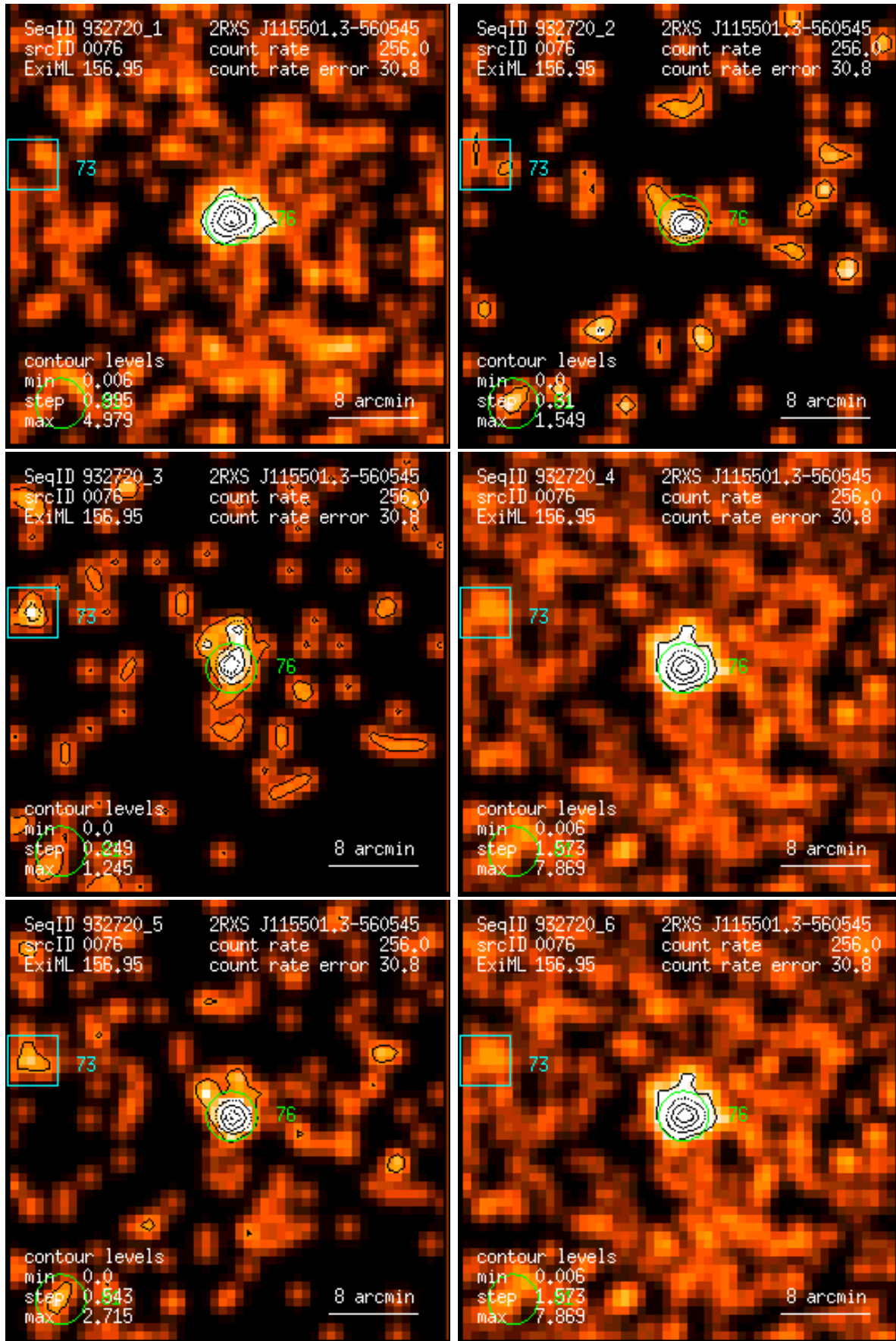
Figure 76: RASS 932720: detection 0076: band rate images, Gaussian filter: (1) PSPC channels 11 – 41, (2) 52 – 90, (3) 91 – 201, (4) 11 – 235, (5) 52 – 201, (6) 11 – 201. Broad band rates in counts/ks. Band rate contour levels in counts/ks/arcmin 2 .
