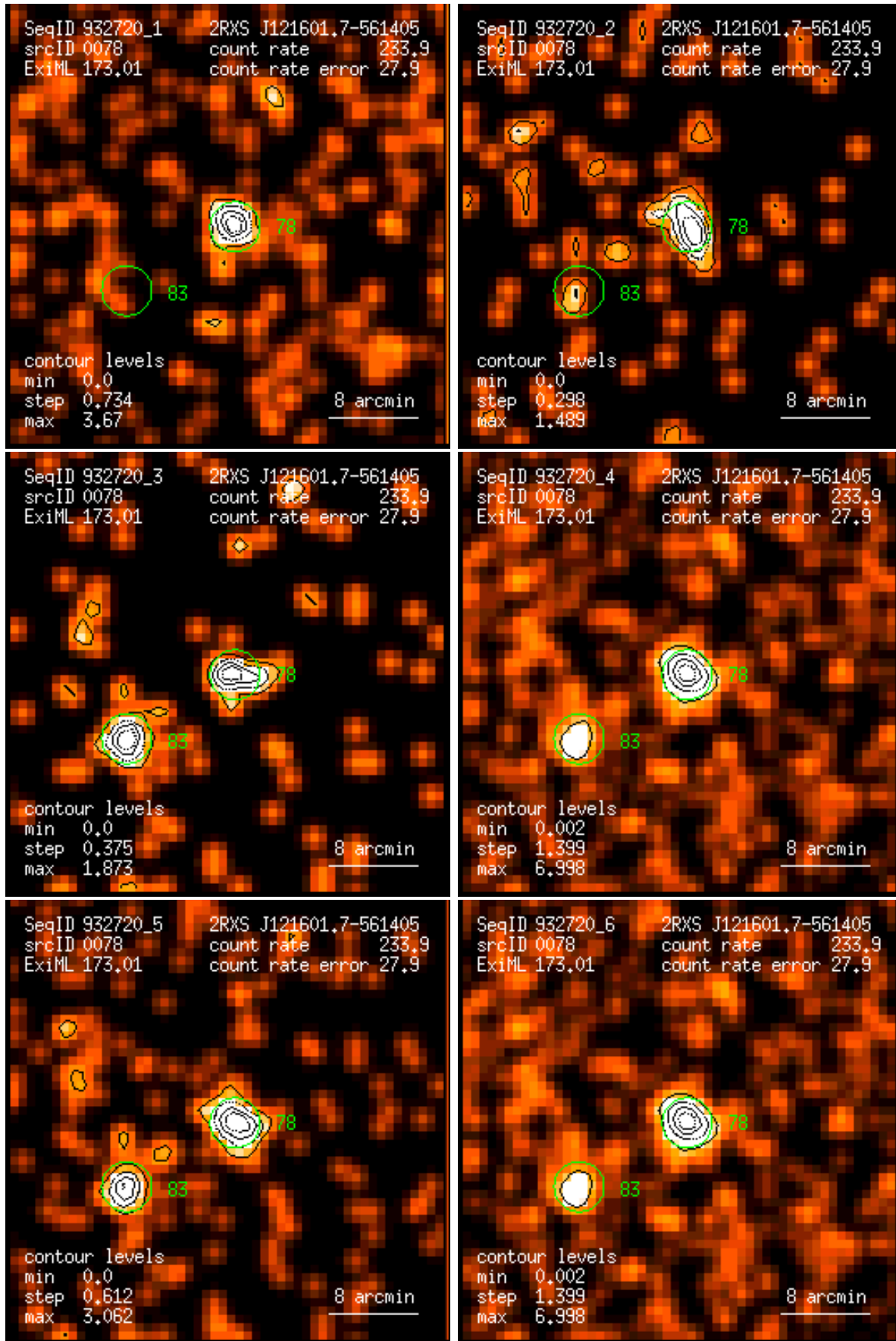
Figure 78: RASS 932720: detection 0078: band rate images, Gaussian filter: (1) PSPC channels 11 – 41, (2) 52 – 90, (3) 91 – 201, (4) 11 – 235, (5) 52 – 201, (6) 11 – 201. Broad band rates in counts/ks. Band rate contour levels in counts/ks/arcmin 2 .
