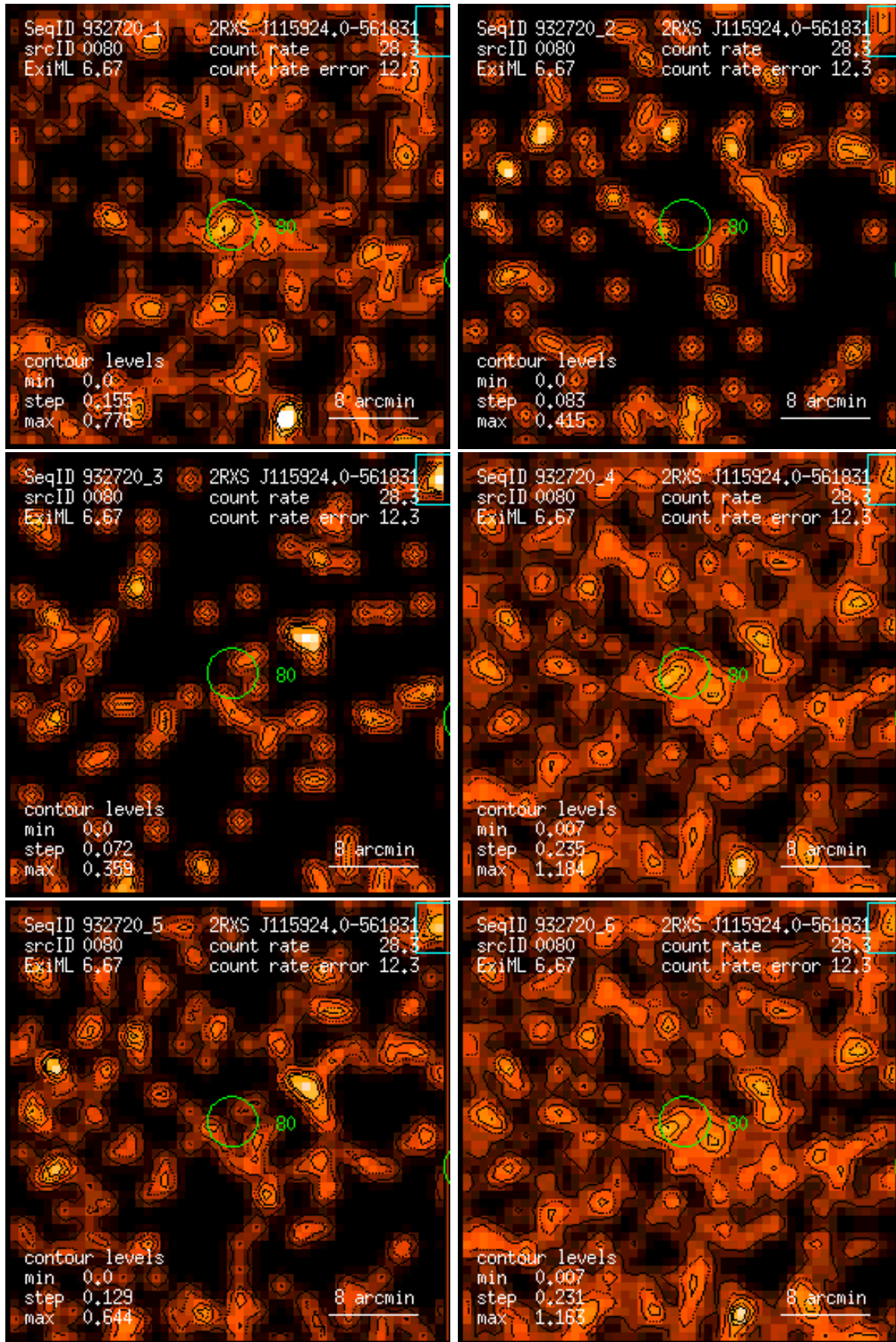
Figure 80: RASS 932720: detection 0080: band rate images, Gaussian filter: (1) PSPC channels 11 – 41, (2) 52 – 90, (3) 91 – 201, (4) 11 – 235, (5) 52 – 201, (6) 11 – 201. Broad band rates in counts/ks. Band rate contour levels in counts/ks/arcmin 2 .
